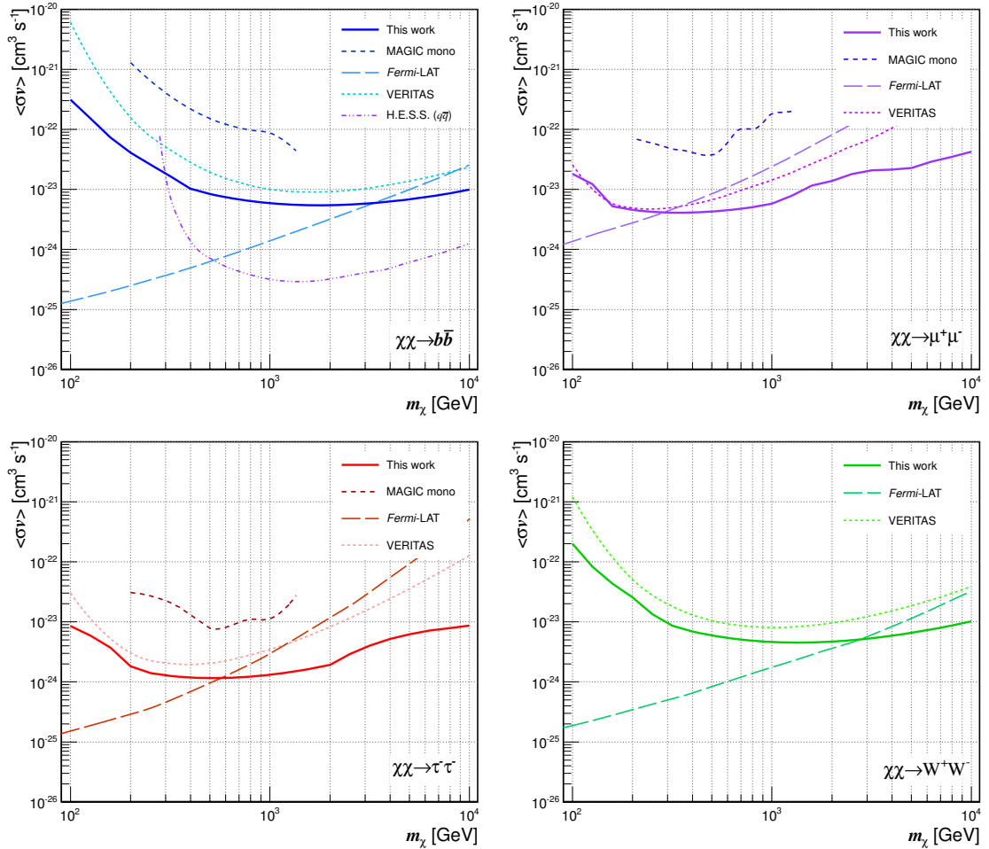
Figure 5: MAGIC upper limits on \langle\sigma v\rangle for different final state channels (from top to bottom and left to right): b\bar{b} , \mu^+\mu^- , \tau^+\tau^- and W^+W^- , from the Segue 1 observations with MAGIC (solid lines, [22]), compared with the exclusion curves from Fermi -LAT (long-dashed lines, [25]), HESS (dot-dashed line, [26]), VERITAS (dotted lines, [27]) and MAGIC in single telescope mode (dashed lines, [28]). Figure taken from [22].
