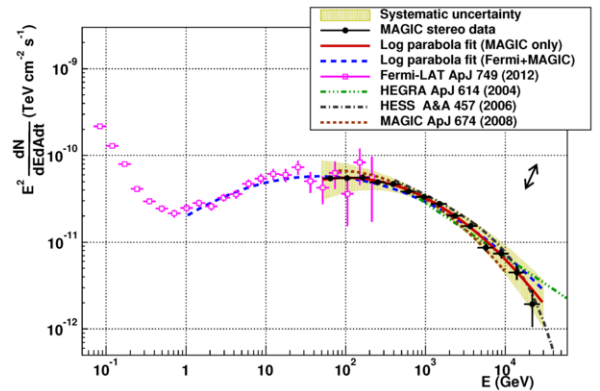
Figure 4: Spectral energy distribution of the Crab Nebula obtained with the MAGIC telescopes, together with the results from other \gamma -ray experiments. The black arrow indicates the systematic uncertainty on the energy scale. The solid red line is the log-parabola fit to the MAGIC data alone, whereas the blue dashed line is a combined fit to the Fermi -LAT and MAGIC data. Figure taken from [13].
