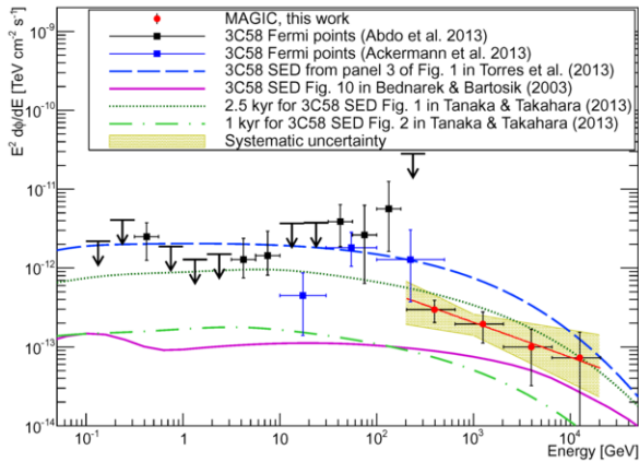
Figure 3: 3C 58 spectral energy distribution in the range between 0.1 GeV and 20 TeV. Red circles are the VHE points reported in this work. The best-fit function is drawn in red and the systematic uncertainty is represented by the yellow shaded area. Black squares and arrows are taken from the Fermi -LAT second pulsar catalog. Blue squares are taken from the Fermi -LAT high-energy catalog. The magenta, clear green dashed-dotted, dark green and blue dashed lines correspond to different models of the source. Figure taken from [10].
