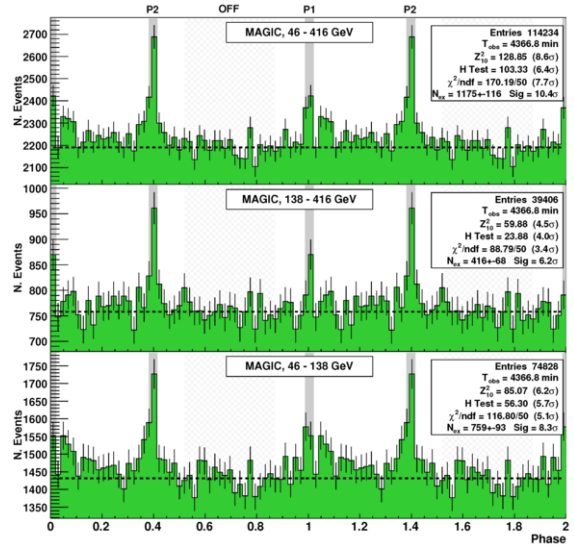
Figure 2: MAGIC folded light curves of the Crab pulsar for our total range in estimated energy and for two separate sub-bins. The shaded areas are the on-phase regions P1_M and P2_M , the light shaded area is the off-region [0.52 – 0.87]. The dashed line is the constant background level calculated from that off-region. Figure taken from [6].
