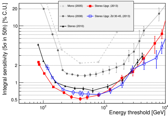
Figure 1: Integral sensitivity of the current MAGIC Stereo system and previous experimental setups, defined as the flux for which N_{\text{excess}} / \sqrt{N_{\text{bgd}}} = 5 after 50 h, and calculated using data from observations of the Crab nebula. Figure taken from [3].
