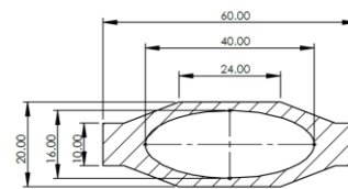
Figure 4: Cross-section of vacuum chambers in straight sections.
