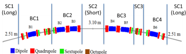
Figure 1: Schematic diagram of SPS-II DTBA cell and sectioned-vacuum chamber.
