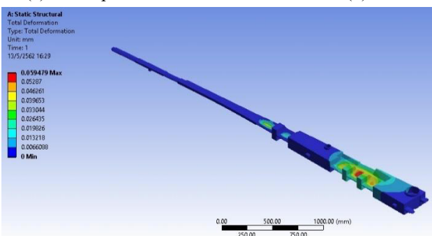
Figure 6: Simulation of the deformation on the chamber BC1 due to the evacuation.
