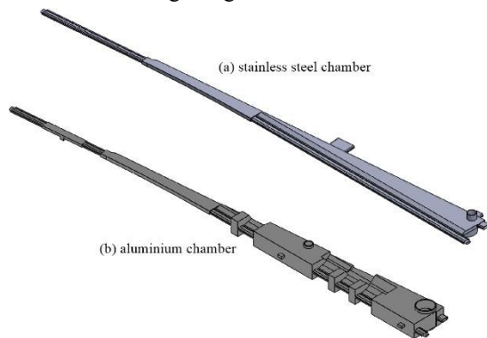
Figure 5: Comparison between stainless steel BC1 chamber(a) and improved aluminium BC1 chamber(b).
