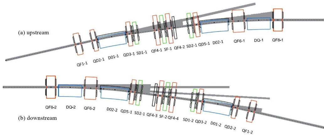
Figure 2: Top-view layout of the upstream (a) and downstream (b) chambers inside the DTBA cell magnets.
