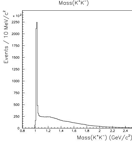
Fig. 1. The K^+K^- sample with no cut on p_T .
