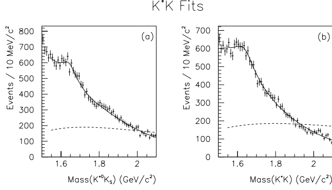
Fig. 5. Fits to K^*K using a Breit-Wigner distribution for the X(1750) region with mass and width fixed from the fit to K^+K^- , a second non-interfering Breit-Wigner distribution around 1630 \text{ MeV}/c^2 , and a quadratic background. The dotted lines are the Monte Carlo efficiencies on a scale from 0 to 20%. (a) K^{*0}K_S with K^{*0} to K^\pm\pi^\mp . (b) K^{*\pm}K^\mp with K^{*\pm} to K_S\pi^\pm .
