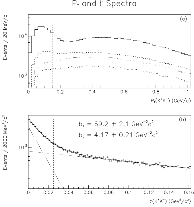
Fig. 2. (a) The K^+K^- p_T spectra. The solid line is the p_T spectrum for the \phi(1020) . The top dotted line is the p_T spectrum for K^+K^- masses between 1640 and 1860 MeV/ c^2 ; the middle is the left sideband (1500–1600 MeV/ c^2 ); and the bottom is the right sideband (1900–2100 MeV/ c^2 ). (b) The t' spectrum for K^+K^- masses between 1640 and 1860 MeV/ c^2 fitted using two exponentials, A_1 e^{-b_1 t'} + A_2 e^{-b_2 t'} . In each plot, the vertical line represents the p_T cut used in this analysis.
