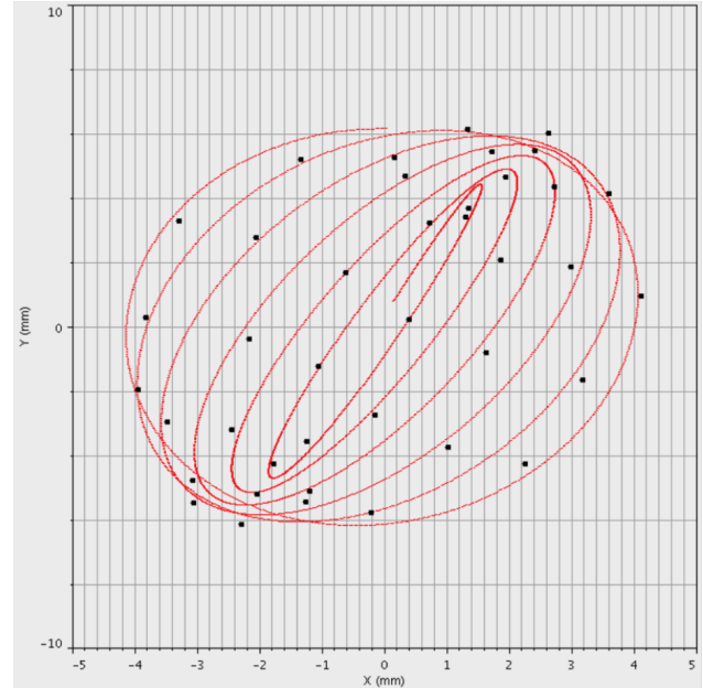
Figure 1: Example of x-y beam position of single minibunch in the Ring measured by single BPM turn by turn.
