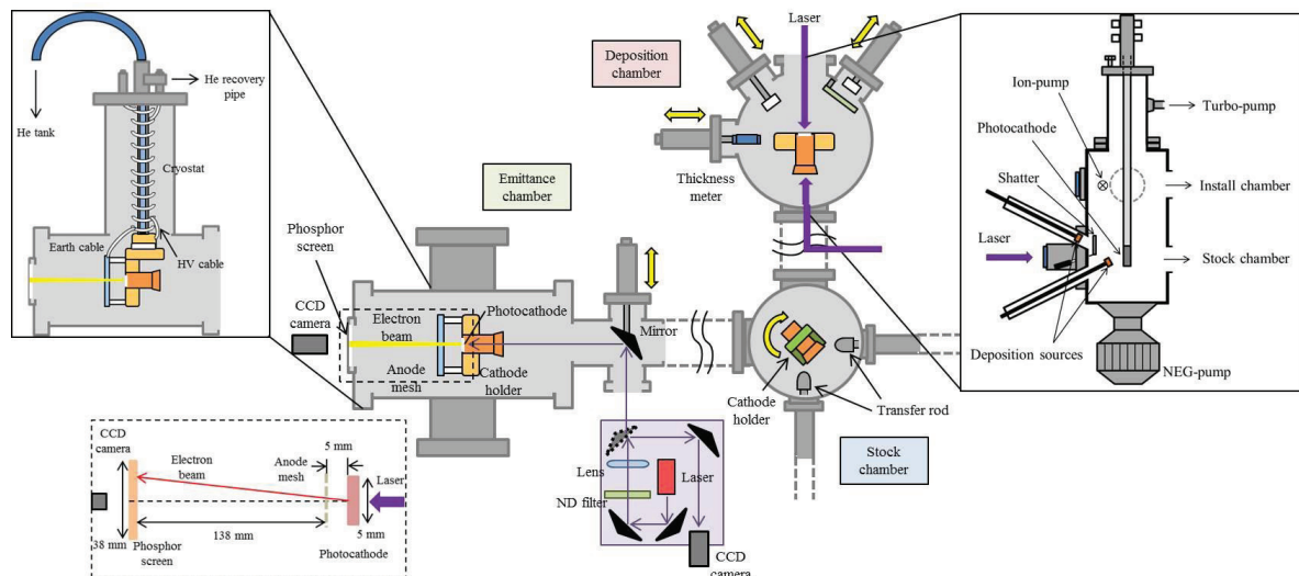
Figure 3: Schematic block diagram of measurement system.
