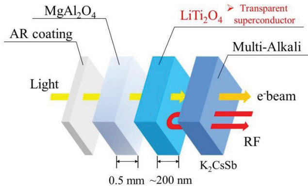
Figure 2: Back-illuminated superconducting photocathode.
