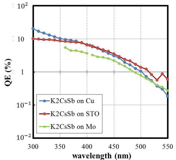
Figure 4: Wavelength dependence of QE.
