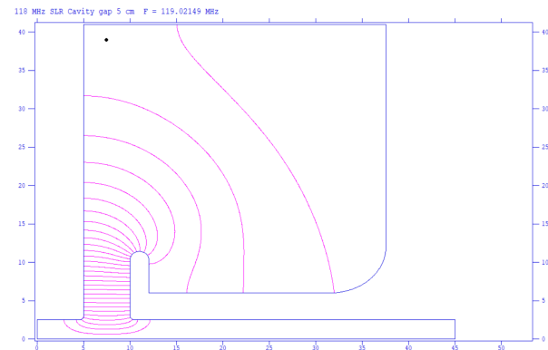
Figure 3: The SPS-II 119 MHz cavity profile.
