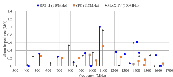
Figure 4: The longitudinal impedance, unloaded, of three cavity designs.
