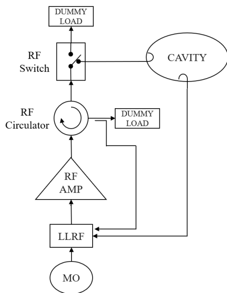
Figure 5: The configuration of RF station.
