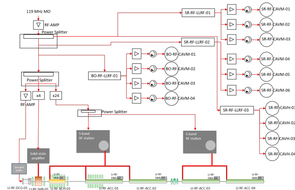
Figure 6: RF frequency distribution diagram.
