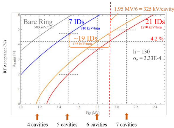
Figure 2: The RF acceptance of the SPS-II storage ring.
