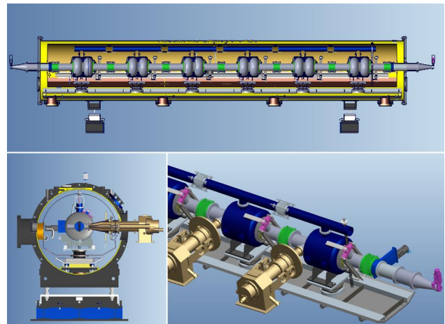
Figure 1: CEPC collider ring 650 MHz 2-cell cavity and cryomodule.
