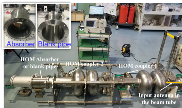
Figure 9: The two 2-cell cavities test bench.
