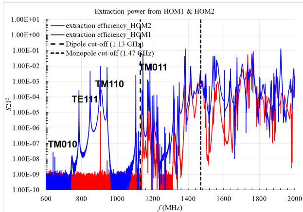
Figure 10: Extraction power efficiency of HOM1 & HOM2.
