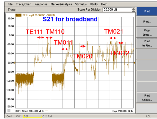
Figure 5: 2-cell cavity HOMs frequencies and passbands.
