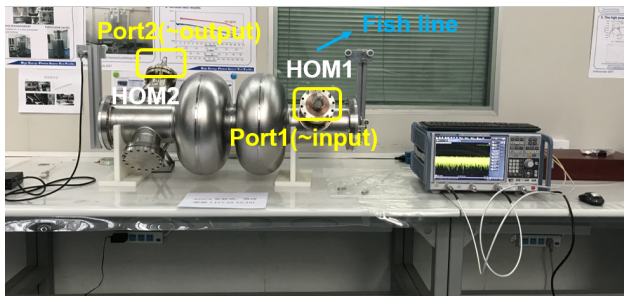
Figure 4: Test bench for HOM measurement.
