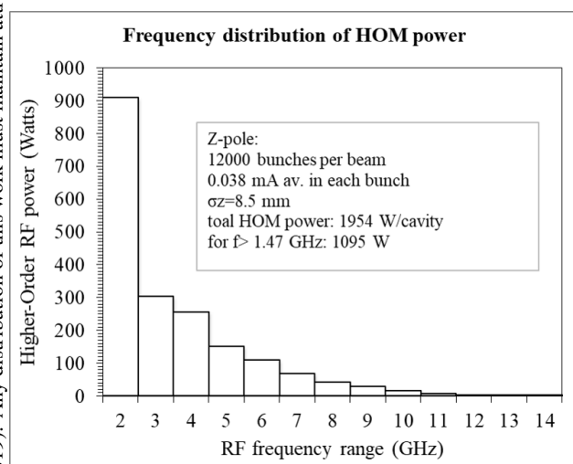
Figure 2: Frequency distribution of HOM power (Z-pole design).
