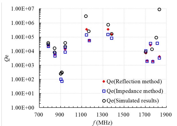
Figure 8: The measured results of Q_e compared with the simulated results.
