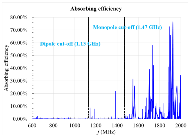
Figure 11: HOM absorber absorbing efficiency.
