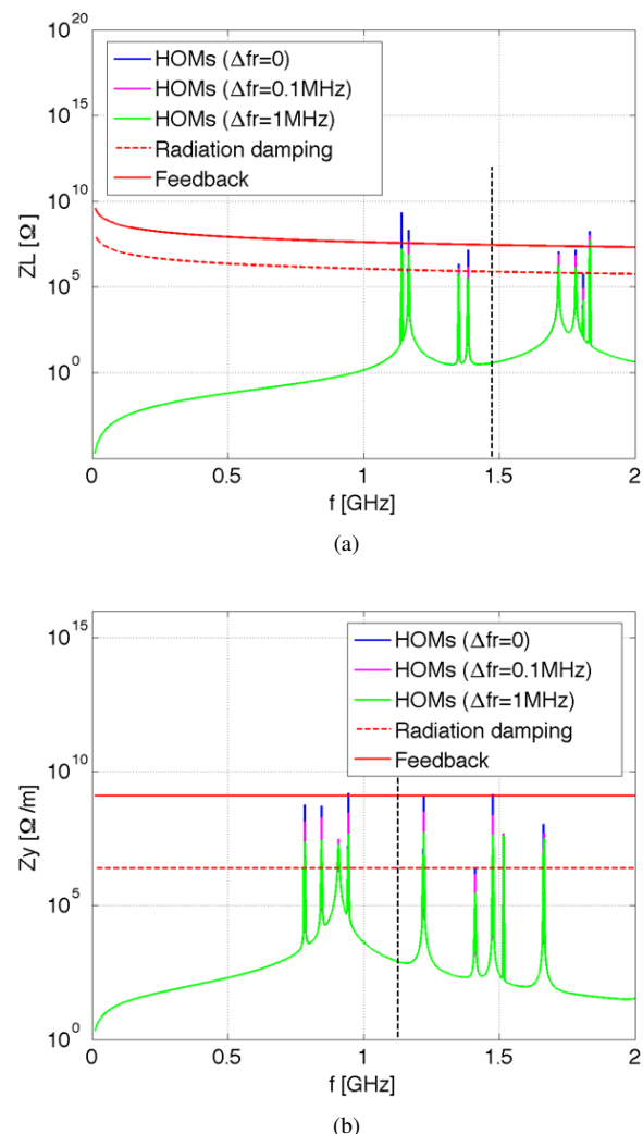
Figure 3: Impedance spectrum of HOMs compared to the threshold determined by radiation damping and feedback damping. (a) Longitudinal HOMs, (b) Transverse HOMs.
