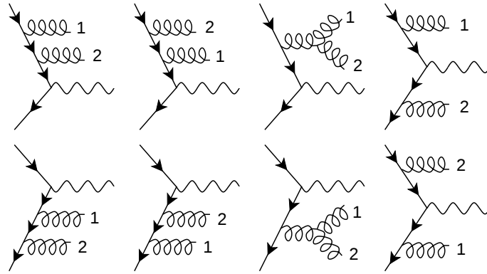
Fig. 1. Feynman graphs for the process q\bar{q} \rightarrow Jgg .
