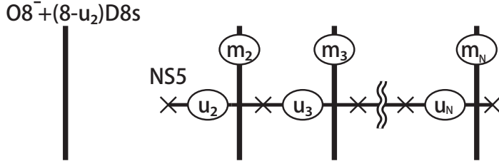
Figure 2.12.: Type I' brane construction of \mathcal{T}_N^{(M9, su)}\{u_i\} [51, 52]. The \times mark represents an NS 5 brane, the horizontal line represents the stack of D6 branes, and the vertical lines represent D8 branes or the stack of O8^- plane and D8 branes. The symbols in the circles are the numbers of the branes there. The m_i D8 branes intersecting with u_i D6 segments supports su(m_i) flavor symmetry. The gauge anomaly cancellation requires m_i = 2u_i - u_{i-1} - u_{i+1} .
