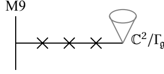
Figure 2.10.: M-theory construction of \mathcal{T}_N^{(M9,g)} with N = 3 .
