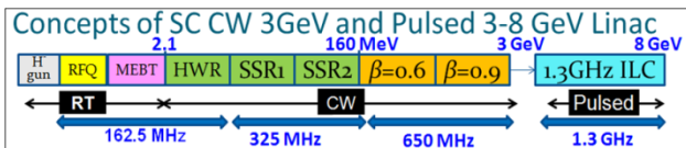
Figure 1: Schematic layout of the Project X accelerator complex
