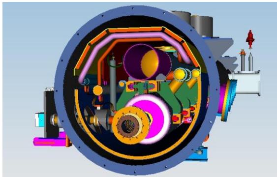
Figure 5: Cross section of 650 MHz cryomodule concept.
