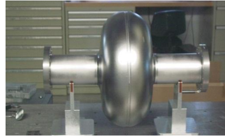
Figure 4: One of six 650 MHz \beta_G = 0.9 cavities form AES. 9cell ILC cavities.
