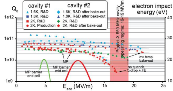
Figure 3: Test results from the JLab prototype cavities. A multipacting simulation is shown on the secondary vertical axis.
