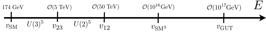
FIGURE 6.1: Diagram showing the different scales of spontaneous symmetry breaking in our example model (see also Eqs.(6.12-6.15)), along with the accidental, approximate flavour symmetries ( U(3)^5 and U(2)^5 ) that arise at low energies.
