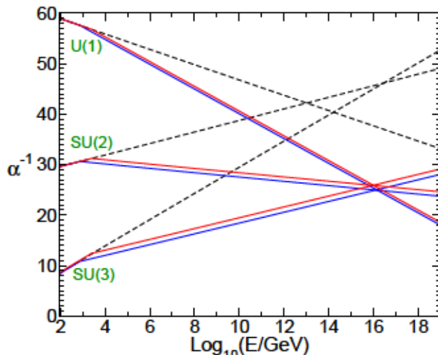
FIGURE 1.4: Two-loop RGE of the inverse gauge couplings \alpha_a^{-1} = 4\pi/g_a^2 in the SM (dashed lines) and the MSSM (solid lines). In the MSSM case, the sparticle masses are
