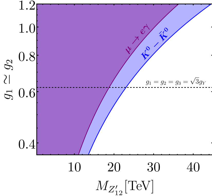
FIGURE 5.1: Parameter space of the high scale breaking, where M_{Z'_{12}} is the mass of the heavy Z'_{12} gauge boson and g_1, g_2 are the gauge couplings of the U(1)_{Y_1} and U(1)_{Y_2} groups, respectively. For simplicity, we assume g_1 and g_2 to be similar, and the non-generic fermion mixing predicted by Model 2 in Section 5.3.4. Shaded regions in the plot depict 95% CL exclusions over the parameter space. The dashed line represents the natural benchmark g_1 \simeq g_2 \simeq g_3 \simeq \sqrt{3}g_Y motivated in the main text.
