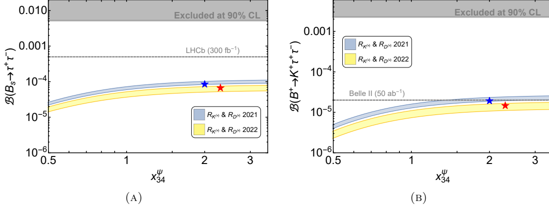
FIGURE 4.13: The branching fractions \mathcal{B}(B_s \rightarrow \tau^+ \tau^-) (left) and \mathcal{B}(B^+ \rightarrow K^+ \tau^+ \tau^-) (right) as a function of x_{34}^\psi , with x_{25}^\psi varied in the range x_{25}^\psi = [0.3, 0.35] ( [0.4, 0.45] ) preferred by R_{K^{(*)}}^{2022} ( R_{K^{(*)}}^{2021} ), obtaining the yellow (blue) band. The rest of the parameters are fixed as in Table 4.5. Current exclusion limits are displayed, along with their future projections. The blue (red) star shows BP1 (BP2).
