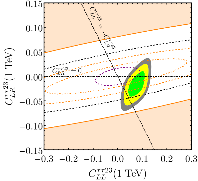
FIGURE 2.5: Parameter space of Wilson coefficients motivated by the U_1 vector leptoquark explanation of R_{D^{(*)}} (see main text). The green, yellow and grey regions represent the 1\sigma , 2\sigma and 3\sigma regions preferred by R_{D^{(*)}} , respectively. Orange contours represent the direct bounds from \mathcal{B}(B_s \rightarrow \tau\tau) , while the black contour represents the indirect bound obtained from \tau_{B_s}/\tau_{B_d} and the purple contour represents the direct bounds from \mathcal{B}(B^+ \rightarrow K^+ \tau\tau) . Solid (dashed) contours denote current (projected) 95% CL exclusions, except for the two projections for \mathcal{B}(B_s \rightarrow \tau\tau) by LHCb: 50 \text{ fb}^{-1} (orange dashed) and 300 \text{ fb}^{-1} (orange dash-dotted). Dash-dotted black lines represent two interesting benchmark scenarios motivated in the main text.
