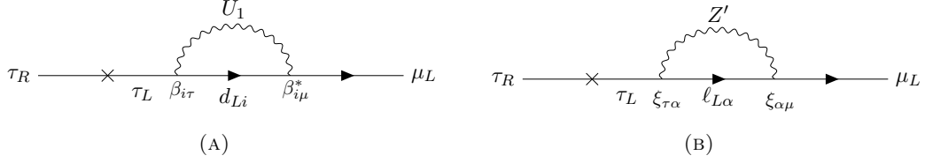
FIGURE 4.10: U_1 (left panel) and Z' (right panel) 1-loop contributions to \tau \rightarrow \mu\gamma . Photon lines are implicit. The index i runs for all down-quarks including vector-like, i.e. d_{Li} = (s_L, b_L, D_{L4}, D_{L5}) , while \alpha runs for all charged leptons including vector-like, i.e. \ell_{L\alpha} = (\mu_L, \tau_L, E_{L4}, E_{L5}) .
