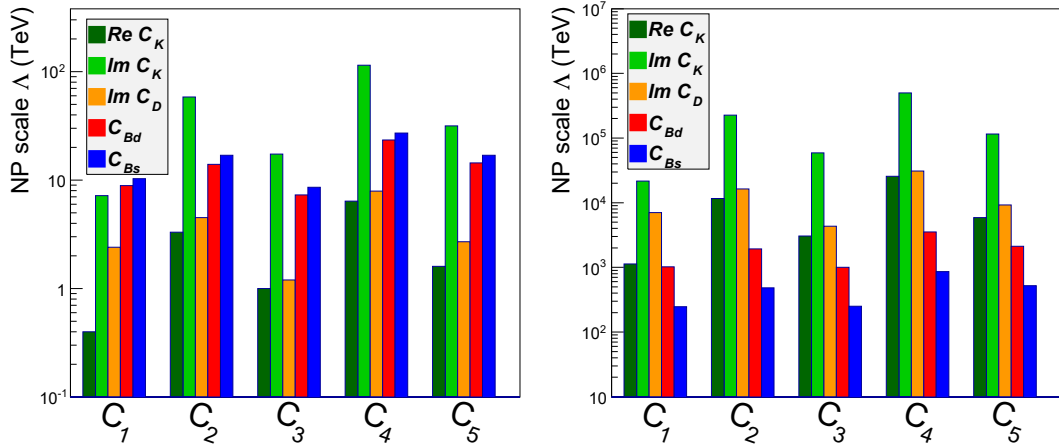
FIGURE 2.4: Summary of the 95% CL lower bound on the NP scale \Lambda for strongly-interacting NP in the U(2)^5 flavour structure (left) and in the general NP scenario (right). Results from all the neutral meson systems are shown. Figure taken from [240].
