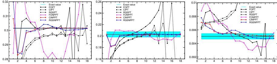
Figure 1: \delta_{W_i}^{(0)} for the weights W_1 , W_6 , and W_{16} calculated for the RM, as functions of the perturbative order up to which the series was summed. The horizontal bands give the uncertainties of the exact values. We use \alpha_s(M_\tau^2) = 0.3186 .
