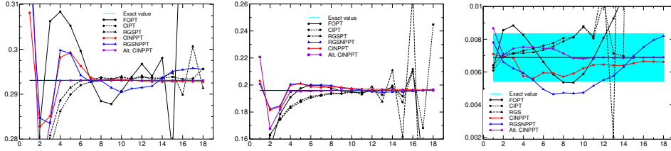
Figure 2: \delta_{W_i}^{(0)} for the weights W_1 , W_6 , and W_{16} calculated for the AM, as functions of the perturbative order up to which the series was summed.
