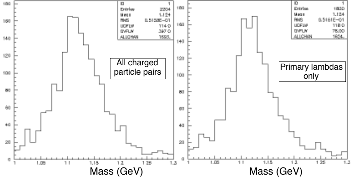
Fig. 9 – Reconstructed \bar{\Lambda} masses for all 2-charged hadron events and for only events with the two hadrons coming directly from the \bar{p} \pm p collision. An energy resolution of 0.60 \sqrt{E} for each hadron and a resolution of 1.0 mrad in their angles is assumed.
