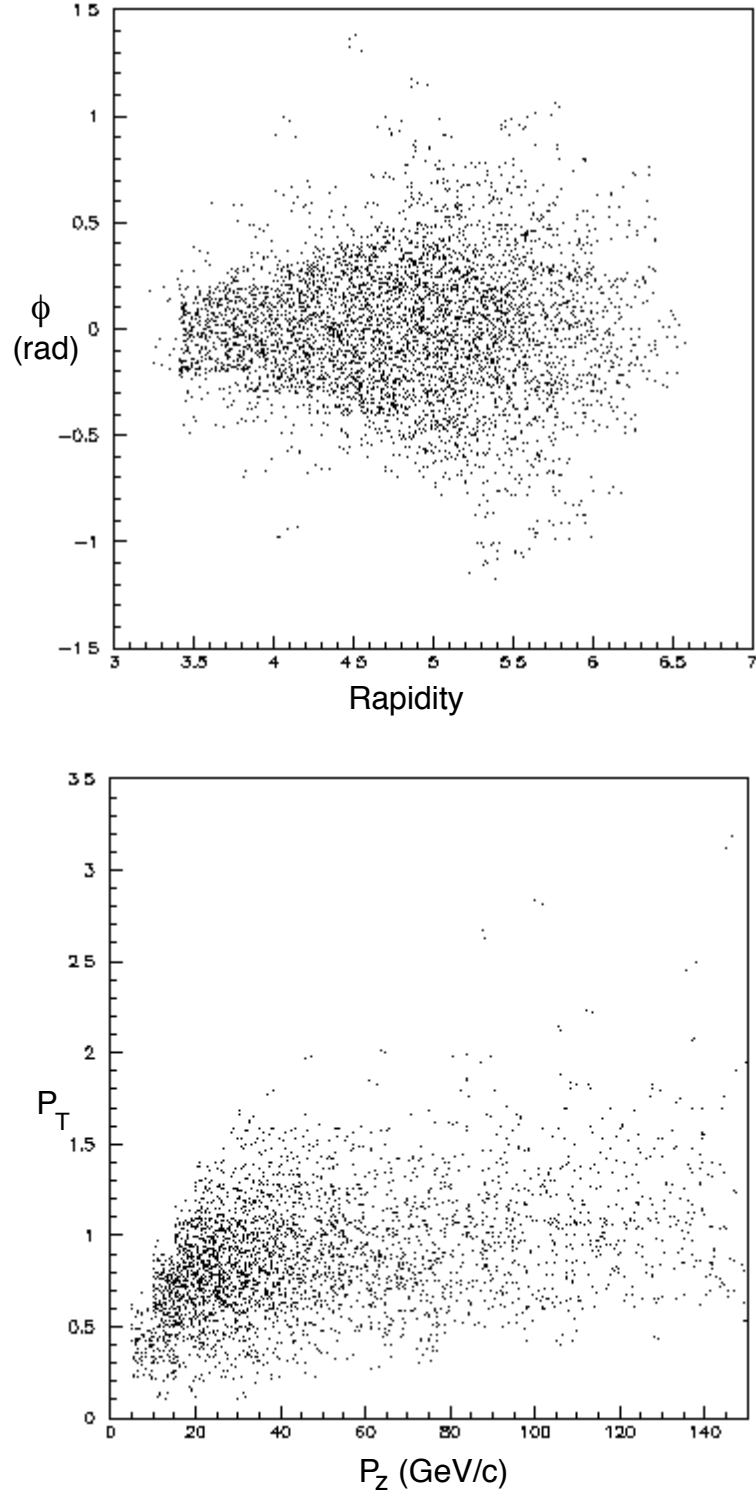
Figure 5 – \phi vs. rapidity and p_T vs. p_z from a PYTHIA/GEANT simulation for positive pions in the outside detector in Fig. 4 with the IP at 20 m. All positive pions coming directly from the IP with E > 5 GeV are plotted.
