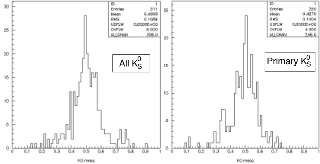
Figure 10—Reconstructed K^0 masses for all 2-charged hadron events and for only events with the two hadrons coming directly from the \bar{p} \pm p collision. An energy resolution of 0.60 \sqrt{E} for each hadron and a resolution of 1.0 mrad in their angles is assumed.
