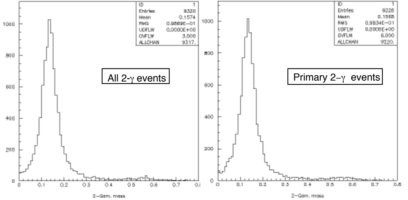
Figure 8—Reconstructed 2\gamma masses for all events with only 2\gamma 's and for 2\gamma events coming directly from the \bar{p} - p collision. An energy resolution of 0.15\sqrt{E} for each \gamma and a resolution in their separation at the detector of 2 cm is assumed.
