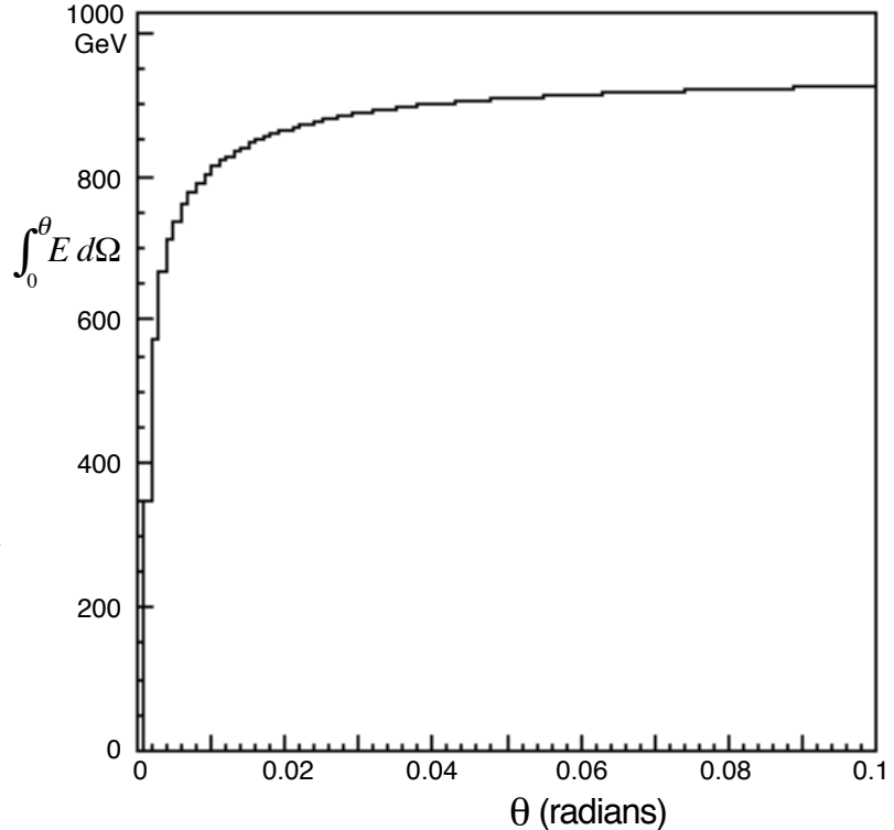
Fig. 1—Integrated visible energy vs. angle for PYTHIA minimum bias events. About 90% of the energy is contained within 14 mrad of the beams.
