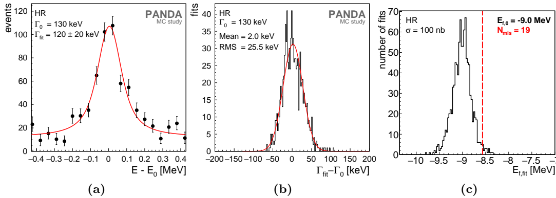
Figure 3: Energy dependent yield distribution (a), distribution of the extracted widths compared to the input value for 1000 toy MC experiments (b) and misidentification fraction for the molecular case (c). [7].
