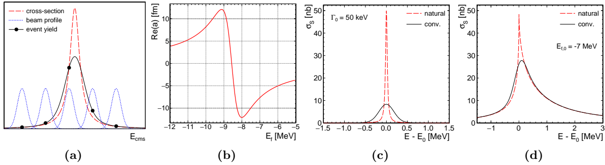
Figure 1: Schematic of a resonance energy scan (a), the functional dependence of the real part of the scattering length on the parameter E_f (b) and two examples for different line shapes in case of a Breit-Wigner resonance (c) and a virtual state (d) [7].
