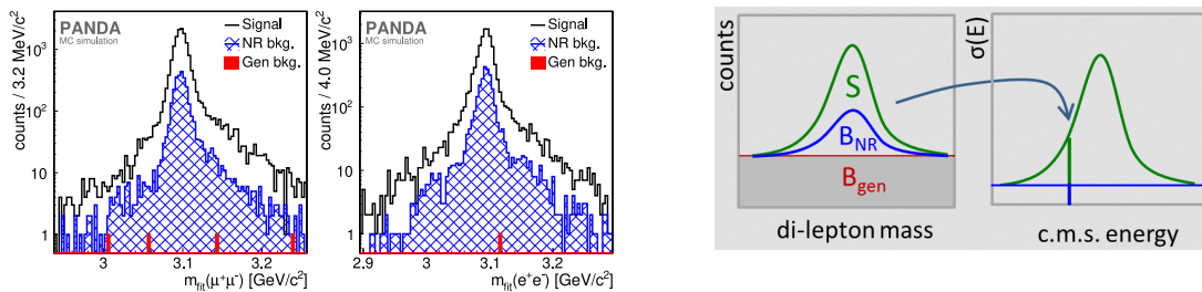
Figure 2: Invariant di-lepton mass after the final selection (left) and scheme of extracting the event yield for each scan point (right) [7].
