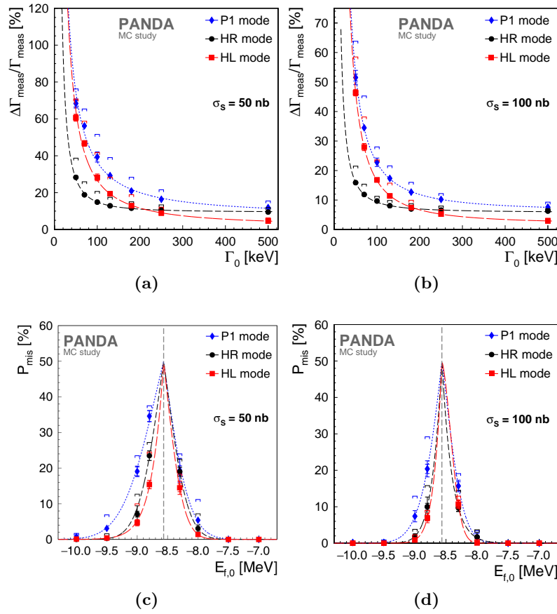
Figure 4: Sensitivity measurements for the Breit-Wigner case study (a)(b) and for the molecule case study (c)(d) for signal cross-sections of 50 nb and 100 nb. The inner error bars represent the statistical and the outer ones the systematic errors. [7].
