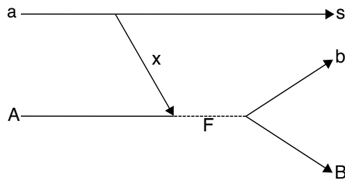
Fig. 1. The diagram describing the TH reaction a + A \rightarrow b + B + s in the QF kinematics, proceeding through the formation of the F = b + B resonant state.
