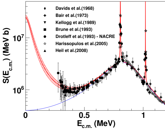
Fig. 3. (Color on-line) R -matrix calculated S(E) -factor of the ^{13}\text{C}(\alpha, n)^{16}\text{O} reaction (red band), obtained using the THM resonance parameters below E_{\text{cm}} = 500 keV and the [30] parameters above, from Ref. [4]. The upper and lower (red) lines delimiting the band mark the range allowed by experimental errors affecting THM data and by the normalization uncertainty. The R -matrix S(E) -factor not including the sub-threshold resonance at -3 keV is displayed by the solid (blue) line. Black symbols are used for direct data normalized as in [30]. Different marks are used for each data set, as specified in the inset. See Ref. [4] for more details.
