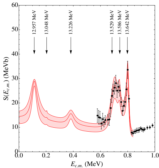
Fig. 2. (Color on-line) THM astrophysical factor of the ^{19}\text{F}(p, \alpha_0)^{16}\text{O} reaction, normalized to the data from [25] above 600 keV, as shown in [26]. The middle solid (red) line marks the recommended S -factor, while the upper and lower solid (red) lines stand for upper and lower limits set by combined statistical, normalization and energy shift error. The solid symbols represent the direct astrophysical factor in [25]. Finally, the arrows mark the ^{20}\text{Ne} states contributing to the S(E) -factor.
