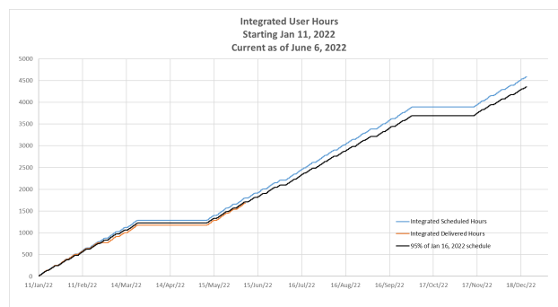
Figure 3: User beam availability and integrated beam delivered for 2022.
