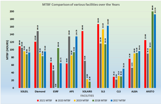
Figure 5: CLS MTBF compared to selected labs.
