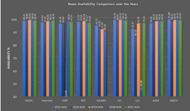
Figure 4: CLS Beam Availability compared to selected labs.
