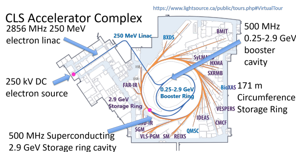
Figure 1: CLS accelerator complex overview.
