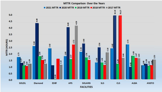
Figure 6: CLS MTTR compared to selected labs.
