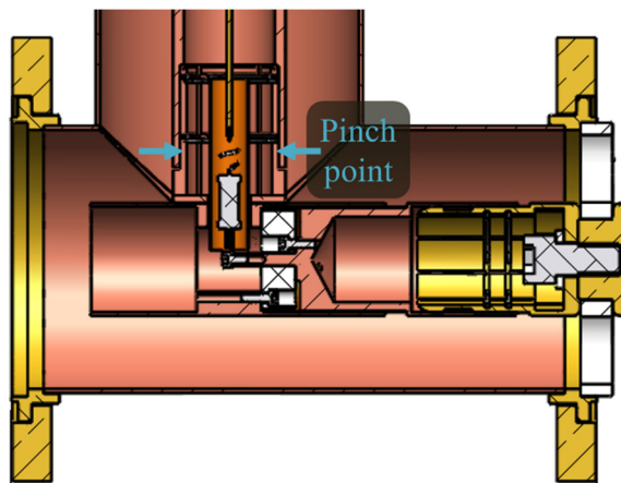
Figure 3: Pinch point on bias tee stub connector.
