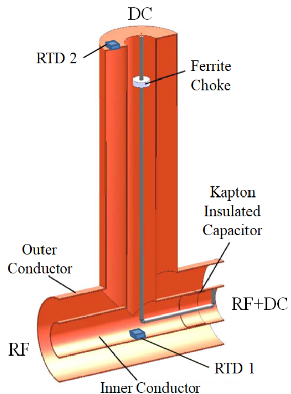
Figure 1: Bias tee concept model.
