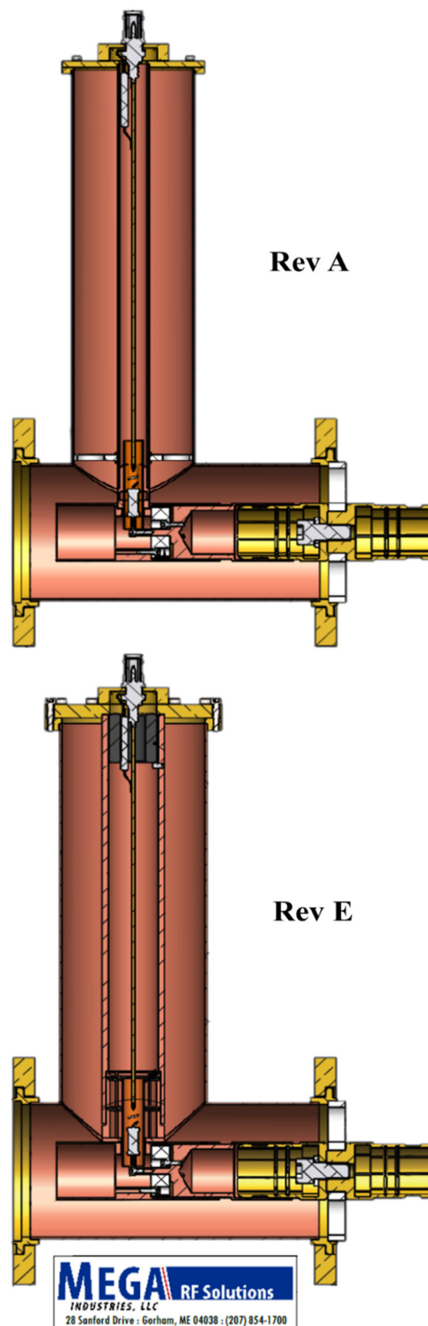
Figure 2: Comparison of cross-sections for Mega Revision A and Revision E tees.
