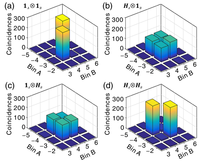
Fig. 4. Coincidences between output frequency bins after the following gates: (a) \mathbb{1} on both photons, (b) H on photon A , (c) H on photon B , (d) H on both photons. Coincidences are collected over 120 s.
