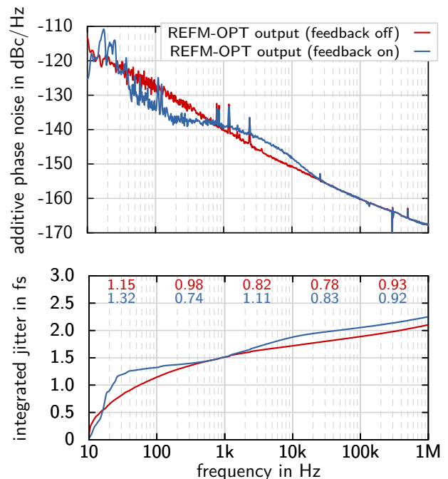
Figure 3: Additive phase noise of the REFM-OPT at the RF station A2M. The measurement was obtained in the accelerator tunnel under operation conditions.
