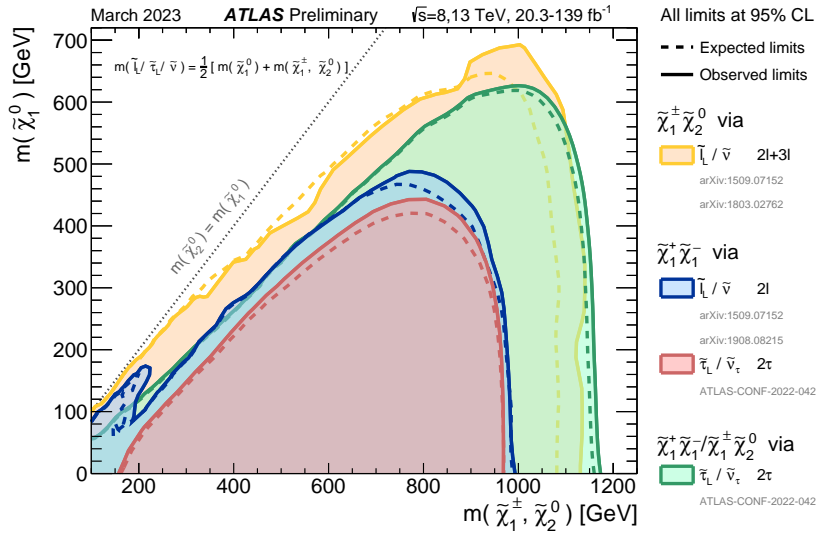
Figure 11: The 95% CL exclusion limits on \tilde{\chi}_1^+ \tilde{\chi}_1^- and \tilde{\chi}_1^\pm \tilde{\chi}_2^0 production with \tilde{\ell} -mediated decays, as a function of the \tilde{\chi}_1^\pm , \tilde{\chi}_2^0 and \tilde{\chi}_1^0 masses. The production cross-section is for pure wino \tilde{\chi}_1^+ \tilde{\chi}_1^- and \tilde{\chi}_1^\pm \tilde{\chi}_2^0 . Each individual exclusion contour represents a union of the excluded regions of one or more analyses.
