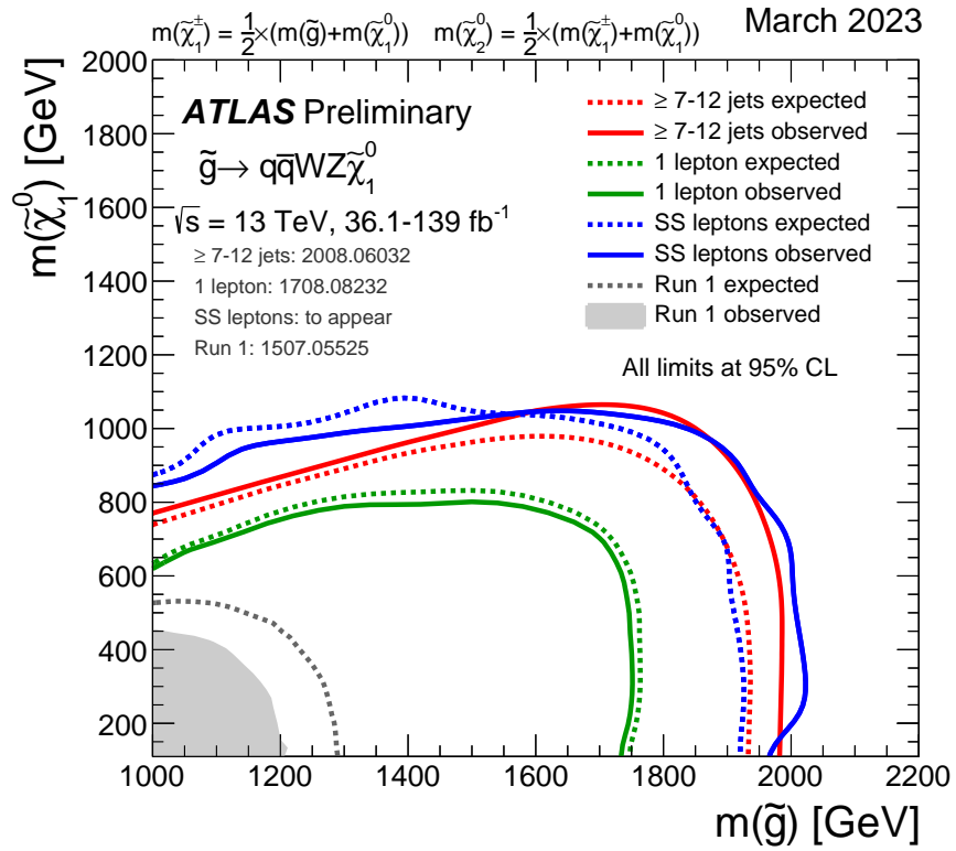
Figure 5: Exclusion limits at 95% CL based on 13 TeV data in the (gluino, lightest neutralino) mass plane for the simplified model where a pair of gluinos are produced, and each decays promptly via the lightest chargino and the second lightest neutralino to a pair of quarks, a W boson, a Z boson, and the lightest neutralino. The assumptions for the masses of the lightest chargino and the second lightest neutralino are reported in the plot. Theoretical signal cross section uncertainties are not included in the limits shown.
