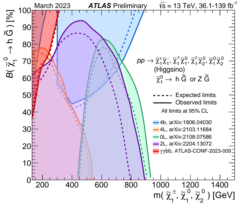
Figure 21: The 95% CL exclusion limits on a general gauge mediation model from 13 TeV data. The model assumes a pure Higgsino NLSP that promptly decays to either Z plus gravitino or Higgs plus gravitino. The limits are displayed as a function of the mass of the nearly mass-degenerate Higgsino multiplet and the branching fraction of lightest Higgsino to Higgs gravitino.
