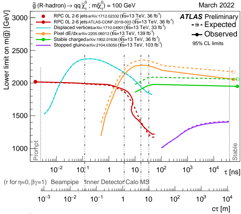
Figure 22: Constraints on the gluino mass-vs-lifetime plane for a split-supersymmetry model with the gluino R -hadron decaying into a gluon or light quarks and a neutralino with mass of 100 GeV. The solid lines indicate the observed limits, while the dashed lines indicate the expected limits. The area below the curves is excluded. For the displaced vertices result the expected and observed limits are identical. For the stopped gluino result the limit extends to larger lifetimes (not quoted here, see reference). The analyses have sensitivity at lifetimes other than those shown, but only the limits at tested lifetimes are shown. The dots represent results for which the particle is assumed to be prompt or stable. In this context, stable means escaping the detector. The displaced exclusion contours from the pixel dE/dx and stable charged particle searches are extrapolated to the stable regime with a straight line.
