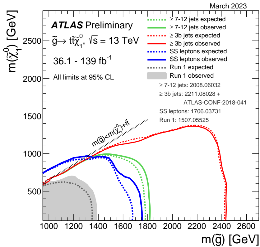
Figure 3: Exclusion limits at 95% CL based on 13 TeV data in the (gluino, lightest neutralino) mass plane for a simplified model where a pair of gluinos decays promptly via off-shell top squarks to four top quarks and two lightest neutralinos. Theoretical signal cross section uncertainties are not included in the limits shown.
