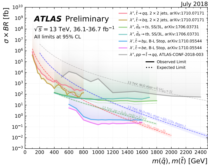
Figure 25: Summary of 95% CL exclusion limits based on 13 TeV data as a function of the squark mass for different simplified models featuring the decay of squarks via R -parity violating couplings. For each line, the squark decay mode is reported in the legend and it is assumed to proceed with 100% branching ratio. Some limits depend on additional assumptions, as described in the references provided in the plot.
