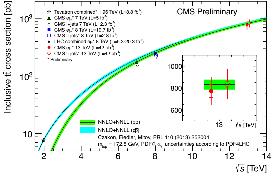
FIGURE 8.8: Top quark pair production cross section in p\bar{p} and pp collisions as a function of center-of-mass energy. The Tevatron combination at \sqrt{s} = 1.96 TeV are displayed, as well as CMS results at 7, 8 and 13 TeV in the dilepton and semileptonic (“ l+l jets”) channels. For the e\mu channel, the LHC combination at 8 TeV is shown. The measurements are compared to the NNLO+NNLL theory predictions.
