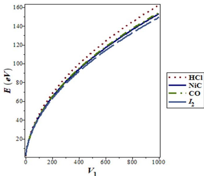
Figure 5. Nonrelativistic ro-vibrational energy versus V_1 for various diatomic. Molecules and \nu = 1 , J = 0 , D = 3 .
