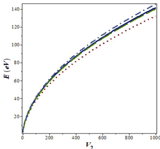
Figure 6. Nonrelativistic ro-vibrational energy versus V_2 for various diatomic. Molecules and \nu = 1 , J = 0 , D = 3 .
