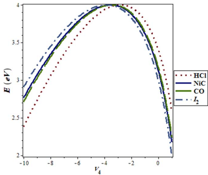
Figure 8. Nonrelativistic ro-vibrational energy versus V_4 for various diatomic. Molecules and \nu = 1 , J = 0 , D = 3 .
