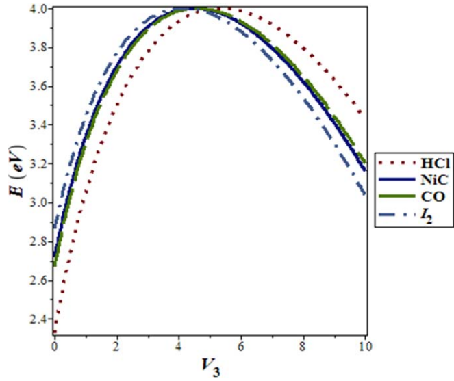
Figure 7. Nonrelativistic ro-vibrational energy versus V_3 for various diatomic. Molecules and \nu = 1 , J = 0 , D = 3 .
