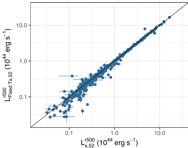
Figure 7. Comparison of luminosity determined using a fixed temperature ( L_{\text{Fixed } T_X,52}^{r_{500}} ) estimated from the luminosity temperature relation (see Section 3.2 for details), to that determined from spectra extracted within r_{500} (see Section 3). The solid black line indicates the 1:1 relation.
