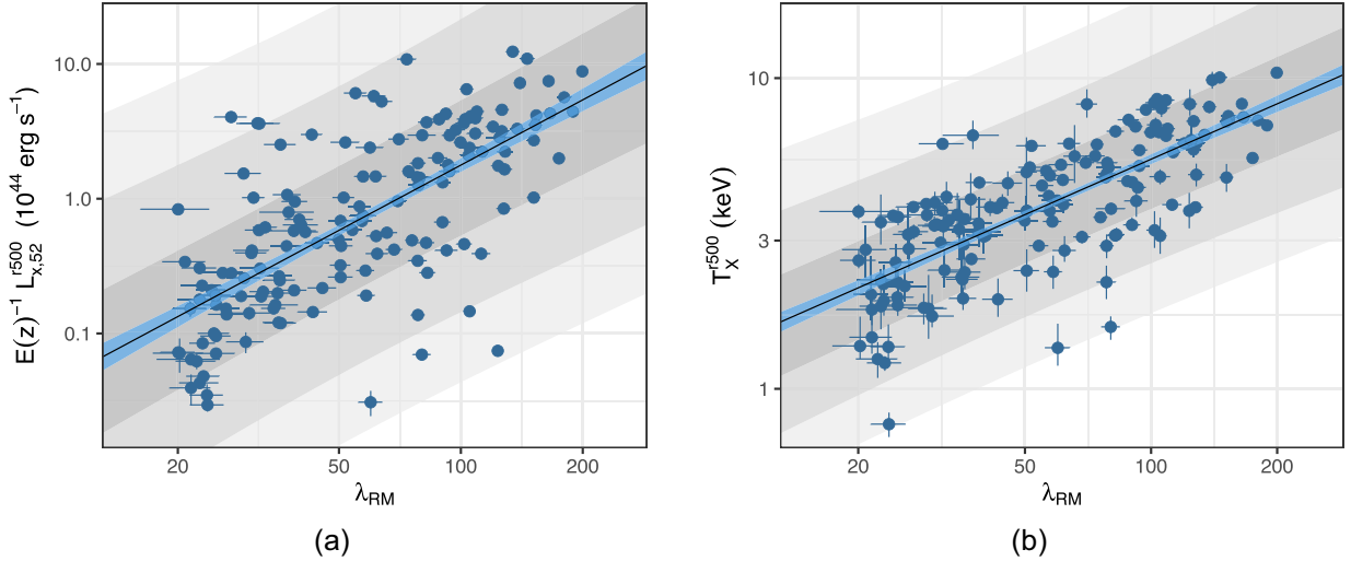
Figure 10. Luminosity–richness (a) and temperature–richness (b) relation of the SDSSRM–XCS T_X ,vol. For each relation, the best fit to the data (see Section 4.2) is represented by the blue solid line, and the light blue shaded region represents the 68 per cent confidence interval of the mean logarithmic relation. The grey bands represent the 1\sigma , 2\sigma , and 3\sigma intrinsic scatter.
