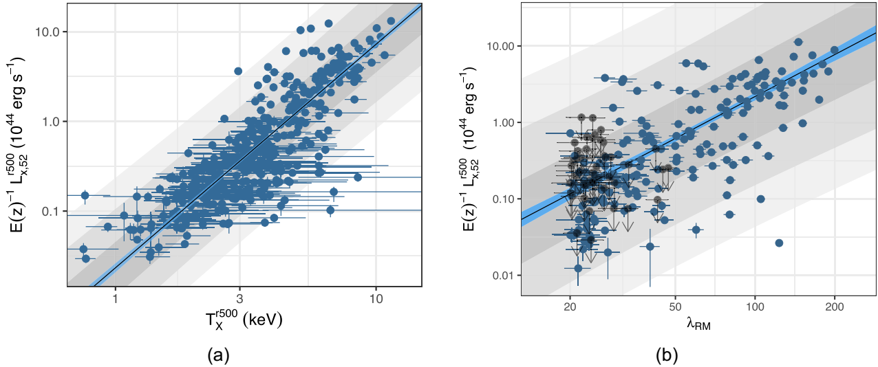
Figure 11. (a) Luminosity–temperature relation of the SDSSRM–XCS _{T_X} sample (blue circles). The best fit to the data is represented by the black solid line, and the light blue shaded region represents the 68 per cent uncertainty. (b) Luminosity–richness relation of the SDSSRM–XCS _{L_X+\text{upper.vol}} subset. Clusters are given by the blue points and luminosity upper limits for SDSSRM–XCS without an XCS detection given by the black circles (and downward arrows). The black solid line represents a fit to the data (including upper limits) with the light blue shaded region highlighting the 68 per cent uncertainty. In each plot, the grey bands represent the 1\sigma , 2\sigma , and 3\sigma intrinsic scatter.
