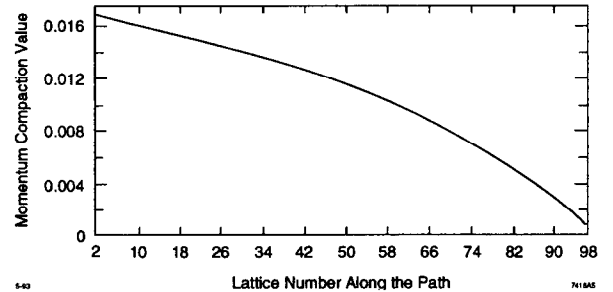
Figure 2. Calculated momentum compaction values along the multi-configuration path.
