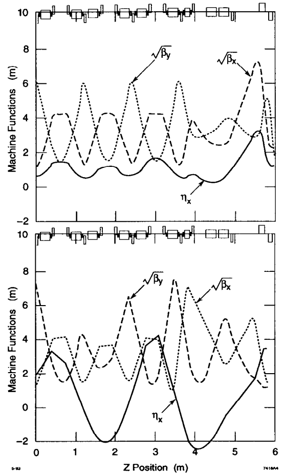
Figure 1. Machine functions of (a) SPEAR low emittance lattice, (b) lattice at the end of the multi-configuration path.
