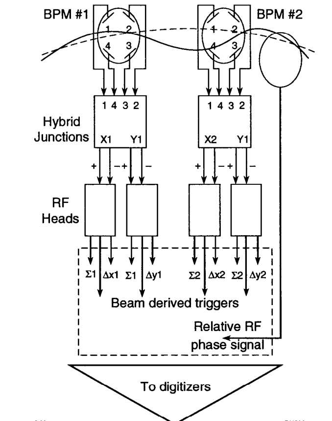
Figure 4. Block diagram of the 6-D PLM system.
