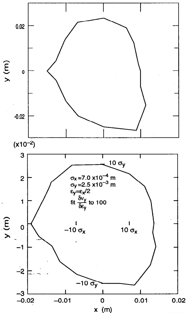
Figure 3. Dynamic aperture of the low momentum compaction lattice used in the direct injection test, (a) tracking without octupoles, and (b) tracking with octupoles.
