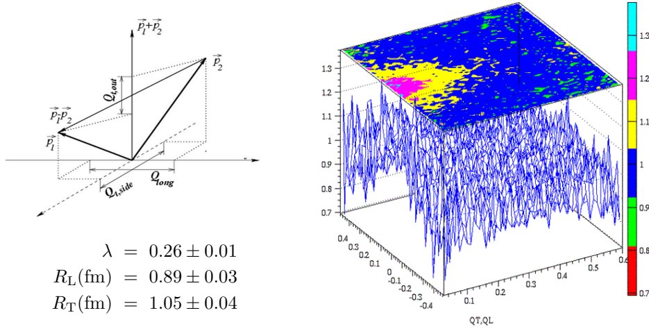
Fig. 3. The LCMS reference system and the two-dimensional BEC function fit results, 5.5 million events.
