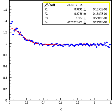
Fig. 2. One-dimensional BEC function.
