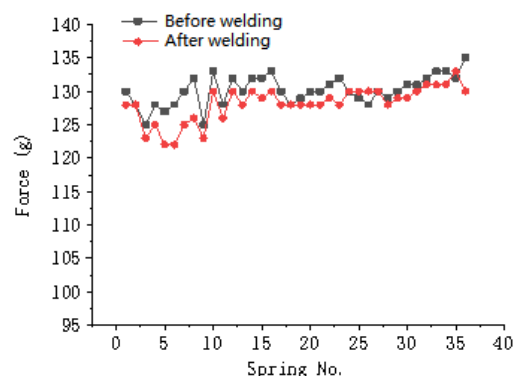
Figure 4: Contact force test results of RF shield bellows prototype.
