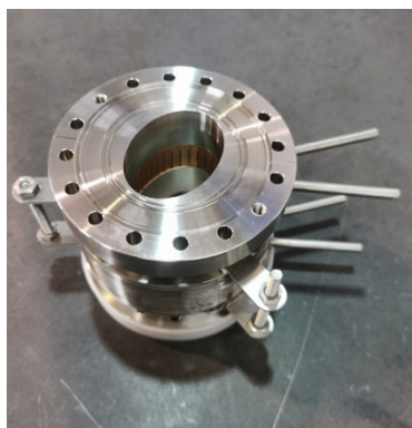
Figure 2: Prototype of RF shield bellows.
