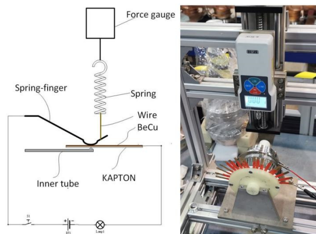
Figure 3: Schematic diagram of the testing device of contact force and its physical photograph.
