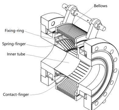
Figure 1: Schematic diagram of the structure of the RF shield bellows.
