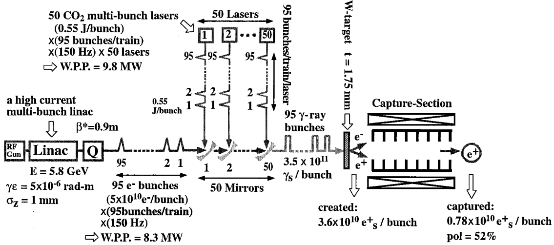
FIG. 5: Schematic design of the JLC polarized positron source.
