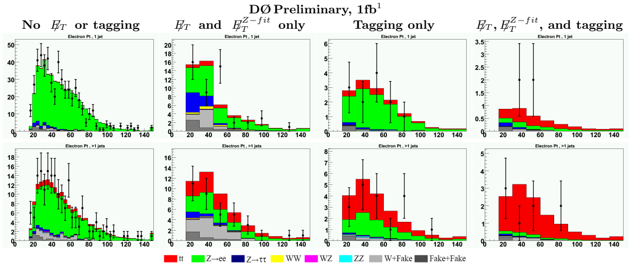
FIG. 4: Electron p_T in e+track. First row is the 1 jet exclusive bin, second row is 2 jet inclusive bin.
