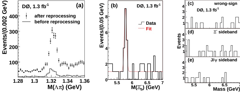
Figure 4: \Xi_b^- observation in D\bar{D} . (a) Invariant mass distributions of the \Lambda\pi^- pair before and after data reprocessing. The reprocessing significantly increases the \Xi_b^- yield. (b) The M(\Xi_b^-) distribution of the \Xi_b^- candidates after all selection criteria. The dotted curve is an unbinned likelihood fit to the model of a constant background plus a Gaussian signal. The (\mu^+\mu^-\Lambda\pi) mass distributions for (c) the wrong-sign background, (d) the \Xi^- sideband, and (e) the J/\psi sideband events. The mass M(J/\psi \Lambda\pi) - M(\mu^+\mu^-) + M_{\text{PDG}}(J/\psi) is plotted for (c) and (d) while the mass M(\mu^+\mu^-\Xi^-) - M(\Lambda\pi^-) + M_{\text{PDG}}(\Xi^-) is plotted for (e).
