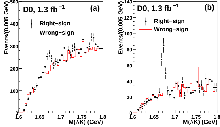
Figure 6: The invariant mass distribution of the \Lambda K pair before (a) and after (b) the BDT selection. Filled circles are from the right-sign \Lambda K^- events while the histogram is from the wrong-sign \Lambda K^+ events without any additional normalization.
