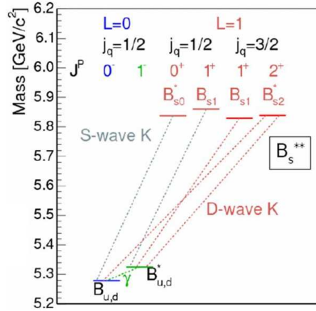
Figure 2: The spectroscopy of the \bar{b}s system. J^P denotes the spin-parity of the state and L the orbital angular momentum.
