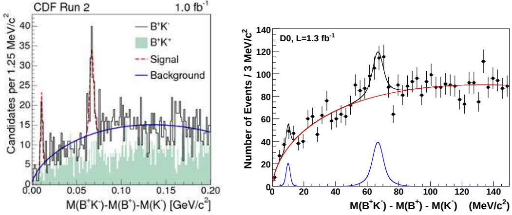
Figure 3: Invariant mass difference for the B_s^{**} candidates in DØ (right) and CDF (left).
