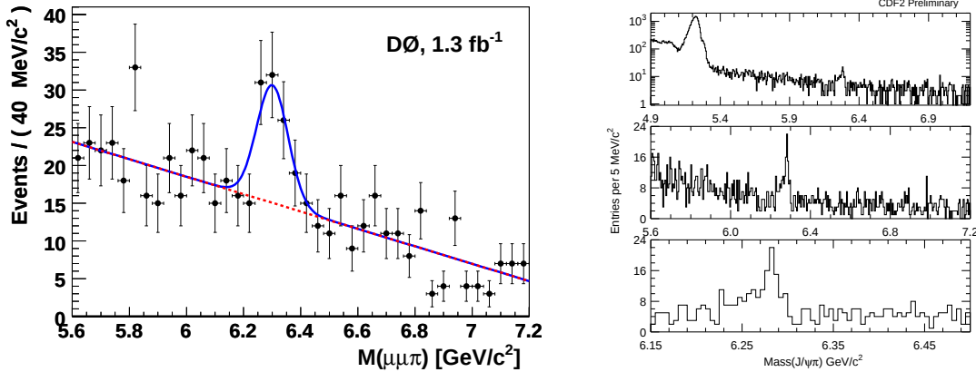
Figure 1: J/\psi\pi invariant mass distribution of B_c^- candidates in D0 (left) and a projection of the unbinned maximum likelihood fit to the distribution is shown overlaid. Right plots shows the B_c^- reconstruction in CDF. Signal in three different mass regions is shown.
