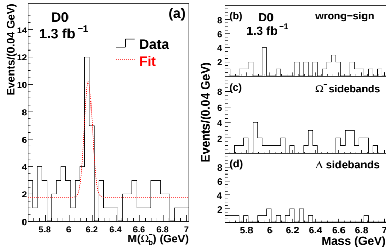
Figure 7: (a) The M(\Omega_b^-) distribution of the \Omega_b^- candidates after all selection criteria. The dotted curve is an unbinned likelihood fit to the model of a constant background plus a Gaussian signal. The mass distributions for the wrong-sign background (b), the \Omega^- sideband events (c), and the \Lambda sideband events (d).
