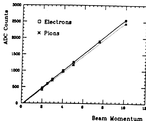
Figure 4. Linearity of calorimeter response with low energy beam.
