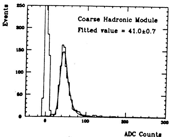
Figure 3. Calorimeter response to 15.9 GeV muons compared to pedestal distribution.
