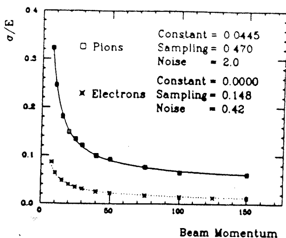
Figure 2. Calorimeter response for electrons and pions.
