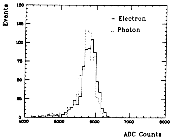
Figure 8. Comparison of photon and electron beams at 25 GeV.
