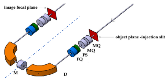
Figure 1: Optical layout of the HRS.
