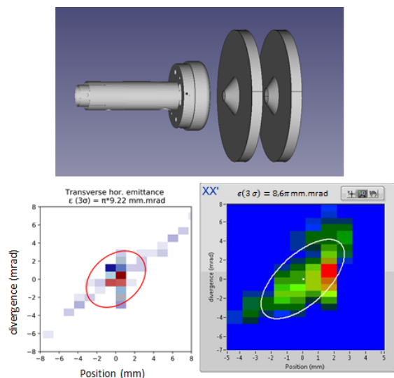
Figure 3: Comparison between simulated and measured beam XX' emittance. Bottom-left: simulated XX' emittance with SIMION. Bottom-right: measured beam XX' emittance. Top: picture of the simulated source.
