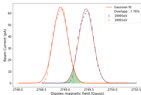
Figure 5: Separation of two beams with a close energy ( \frac{\Delta E}{E} = 1/5000 ). The beams have been separately scanned with the dipoles through the final slits of the HRS, and their intensity monitored with the Faraday cup right after the slits. A Gaussian fit of the beams gives the beam separations and their respective standard deviation, leading to an estimation of the resolution.
