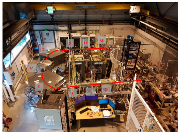
Figure 2: Picture of the HRS mounted at CENBG.
