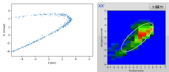
Figure 4: Comparison of the simulated (left) and measured (right) beam emittance at the end of the HRS. This have been simulated with COSY and confirmed by Zgoubi. This figure has been obtained by turning off the last doublet of quads in the beamline so that the beam is large enough to be measured. The tail on the left of the simulated emittance also disappears when a binning and a threshold are applied on the simulated data as for the experimental data.
