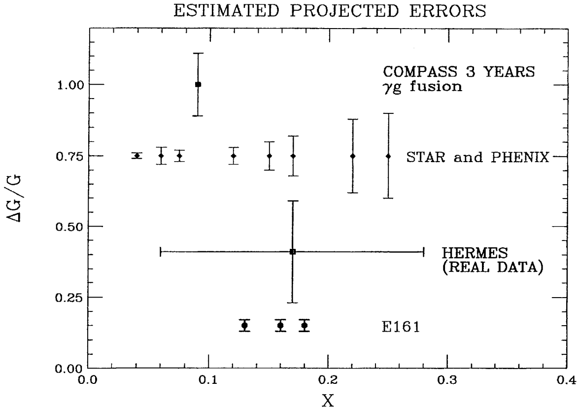
Figure 3: Estimated accuracy of \Delta G/G measurements. Each data set is arbitrarily shifted on the y-axis.
