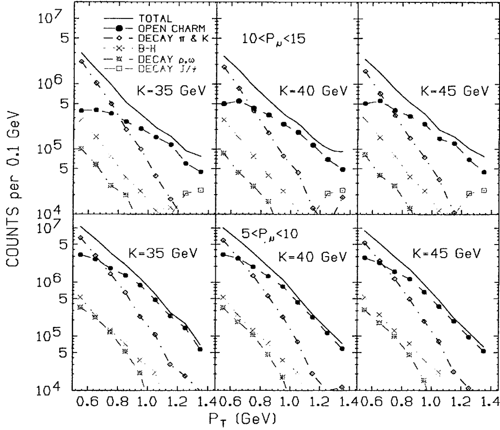
Figure 2: Expected single- \mu events in counts per 0.1 GeV versus p_T for three beam energies k = 35, 40, 45 GeV. Top row: 10 < p_\mu < 15 GeV; bottom row: 5 < p_\mu < 10 GeV; total (solid line), open charm (solid dots), \pi and K decay (diamonds), Bethe-Heitler (crosses), J/\psi (squares), \eta, \rho, \omega, \phi decays (stars).
