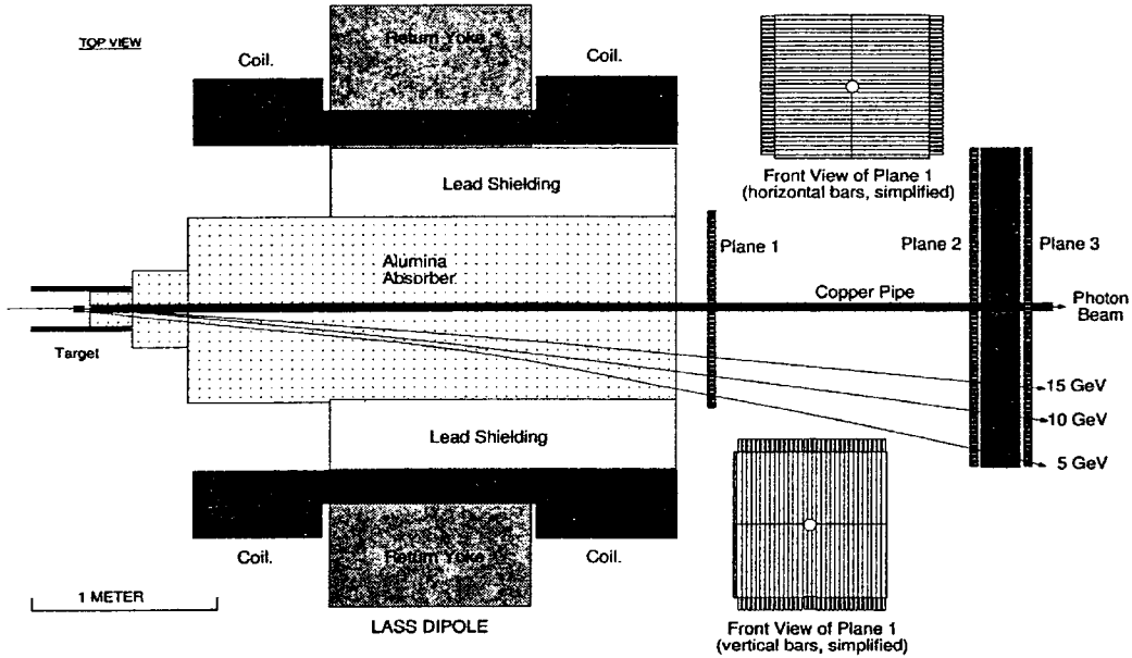
Figure 1: Muon spectrometer for E161. Decay muons are studied by removing some of the shielding following the target.
