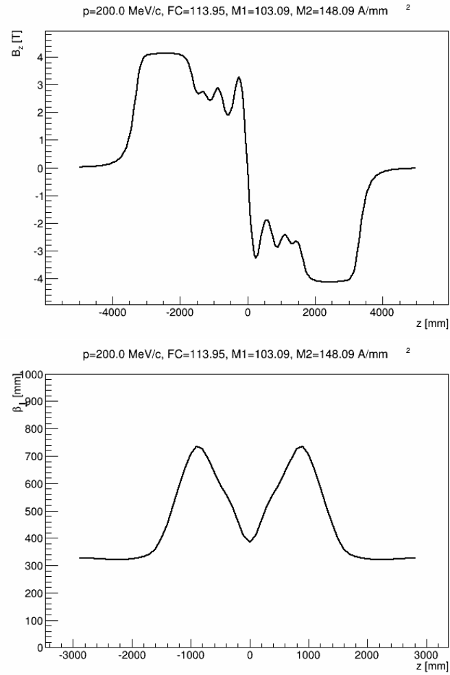
Fig. 1: (Top) Example magnetic field on axis and (bottom) corresponding matched \beta function.
