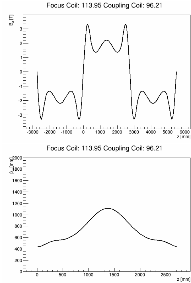
Fig. 3: (Top) Example magnetic field on axis and (bottom) corresponding matched \beta function.
