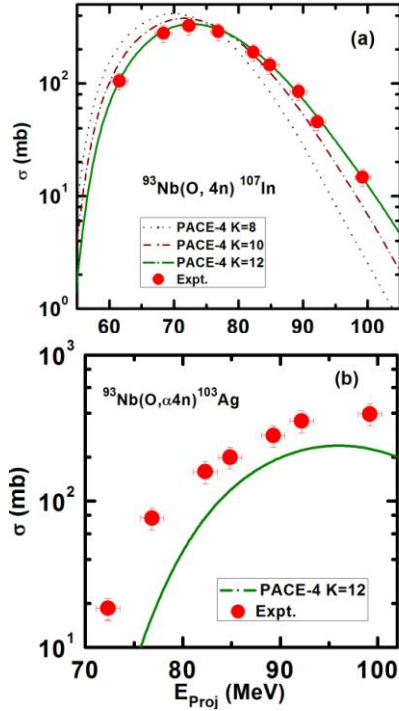
Fig.1: Experimentally measured EFs of evaporation residues ^{107}\text{In}(4n) , and ^{103}\text{Ag}(\alpha 4n) along with PACE-4 predictions.
