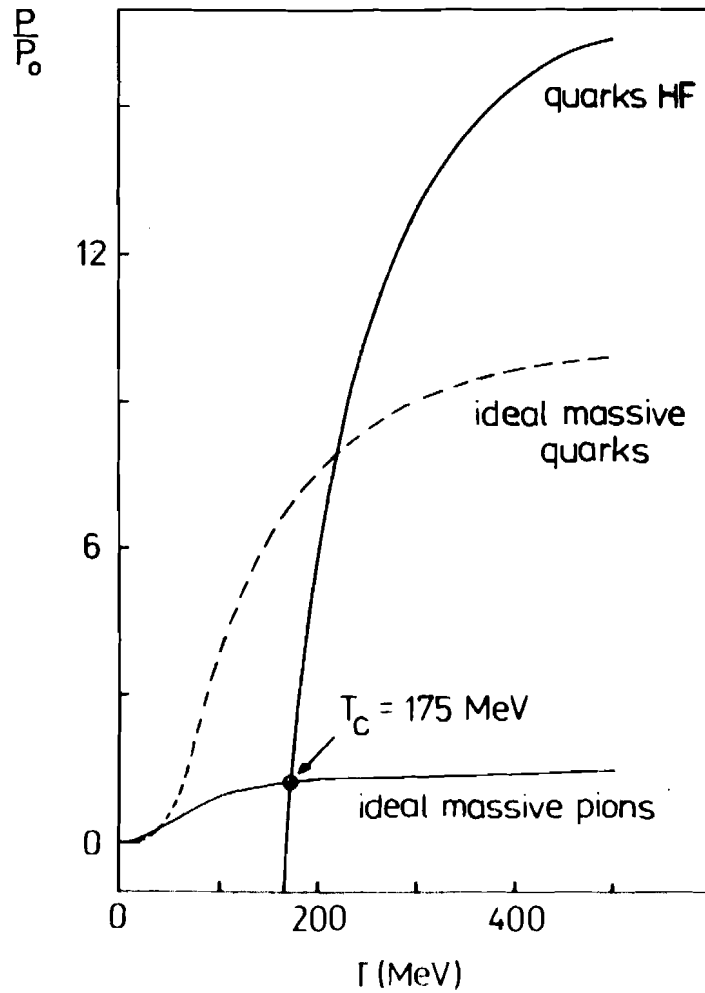
Fig. 1. The pressure of non-interacting massive pions and interacting massive quarks within the Hartree approach as a function of the temperature. The normalization parameter for the pressure is given by p_0 = T^4 \pi^2/45 . To show the influence of the Hartree shift the non-interacting massive quark contribution is also displayed.
