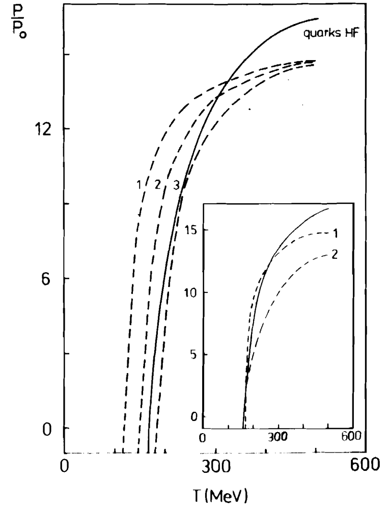
Fig. 2. Comparison between the string-Flip model (Full line) and the first order perturbative QCD bag model (broken lines) with \Lambda = 100 MeV. The values of B_0^{uv} are 145, 190 and 235 MeV for the curves 1, 2 and 3, respectively. The inset shows two different sets of the string-Flip model with \Lambda = 100 MeV, B_0^{uv} = 219 MeV (curve 1) and \Lambda = 273 MeV, B_0^{uv} = 173 MeV (curve 2), respectively.
