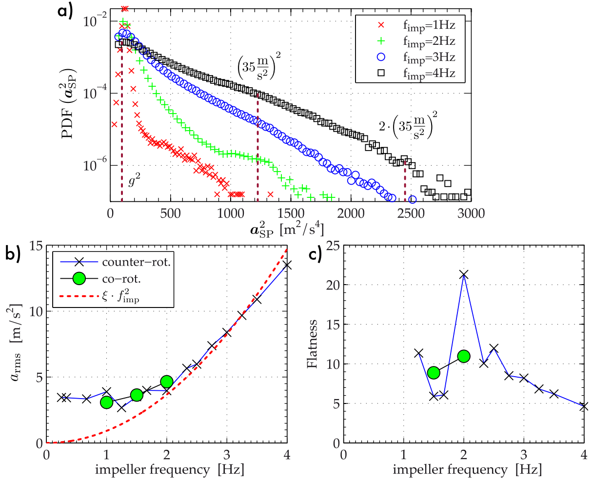
Figure 5. Moments of \mathbf{a}_{trans} . (a) PDF ( a_{SP}^2 ) at different impeller frequencies. The three vertical lines mark gravity and the saturation of one or two accelerometer axes. (b), (c) The rms and fourth moment of \mathbf{a}_{trans} as a function of the impeller frequency. Dimensional analysis suggests a scaling a_{rms} \propto f_{imp}^2 , which is illustrated by the red dashed line in (b). Deviation from the scaling at f_{imp} \lesssim 1 Hz stems from contacts of the particle with walls and impellers.
