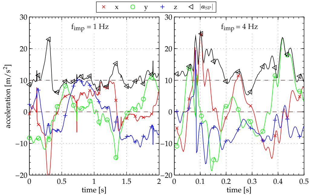
Figure 3. Sample acceleration time-series, \mathbf{a}_{\text{SP}}(t) , with the impellers counter-rotating at f_{\text{imp}} = 1 Hz (left) and f_{\text{imp}} = 4 Hz (right). Both samples last two integral times T_{\text{int}} .
