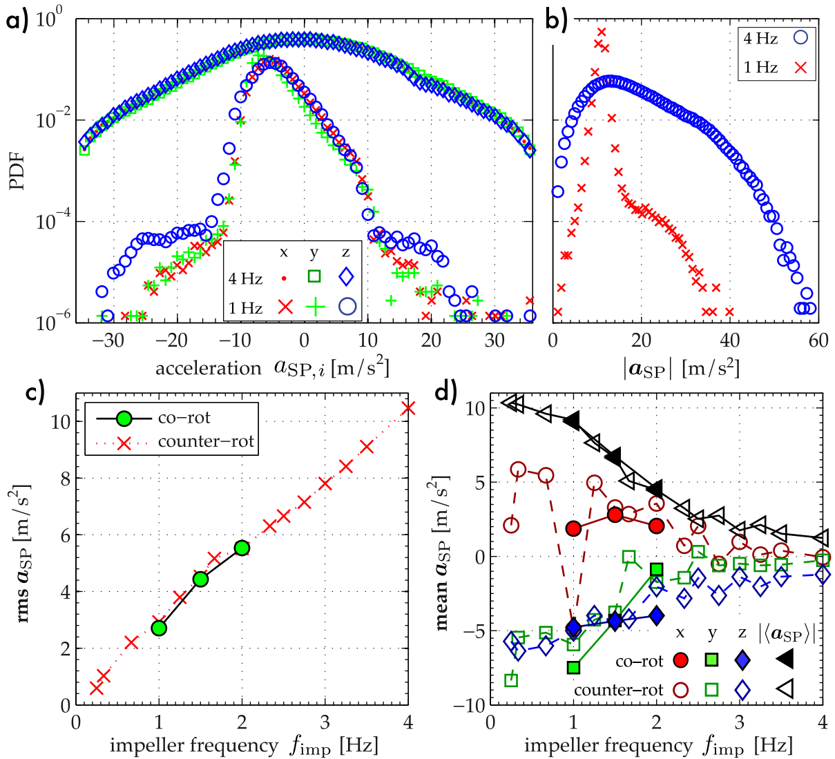
Figure 4. Top: probability density functions (PDFs) of (a) the components and (b) the norm of the acceleration a_{SP} for two different impeller frequencies. For readability, the PDFs of acceleration components at 4 Hz have been arbitrarily shifted. Bottom: evolution of (c) \text{rms } a_{SP} and (d) \langle a_{SP} \rangle with the impeller frequency f_{\text{imp}} ; filled symbols indicate co-rotating impellers. In all cases the particle explored the flow for a sufficient amount of time for the statistics to converge. In good agreement with equation (2), |a_{SP}| continuously decreases from 1g to 0g as the impeller frequency increases.
