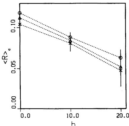
Fig. 6. Average curvature at the phase transition for N_4 = 4000(\bigcirc) , 9000(\triangle) and 16000(\times) .
