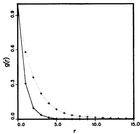
Fig. 15. The spin-spin correlation function g(r) (defined by (3.14)) as a function of the geodesic distance r for \beta = 0.5 (full drawn curve) and \beta = 0.8 (dotted curve), k_1 = 3.7 and N_3 = 4000 . The best estimate of the critical value of \beta is: \beta_c = 0.85
