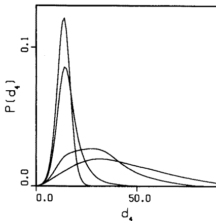
Fig. 9. Distribution of the d_4 distances for h = 0 and \kappa_2 = 1.0, 1.1, 1.2 and 1.3 .
