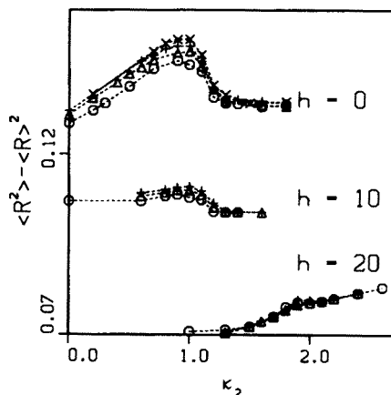
Fig. 4a. \langle R^2 \rangle - \langle R \rangle^2 as a function of \kappa_2 for h = 0, 10 and 20 and N_4 = 4000(\circ) , 9000(\triangle) , 16000(+) and 32000(\times) .
