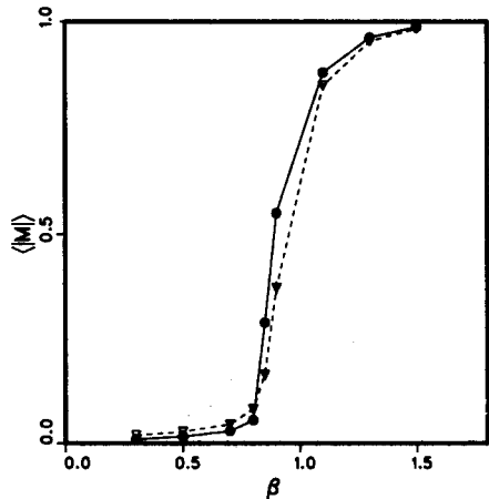
Fig. 11. The magnetization |\sigma| (defined by (5.6)) as a function of \beta in the “cold” phase ( \kappa_1 = 4.4 ) for N_3 = 4000 ( \Delta ) and N_3 = 10000 ( \circ ).
