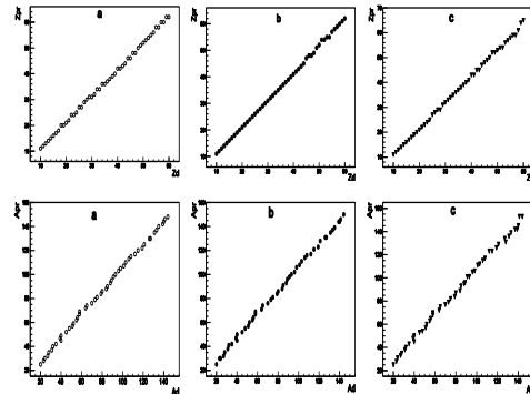
Fig. 1. Top panel: The reconstructed charge of the fissioning fragments: a) at E=18 A MeV, b) at E=20 A MeV and c) at E=25 A MeV. Bottom panel: the reconstructed mass of the fissioning fragments at the same energies.
