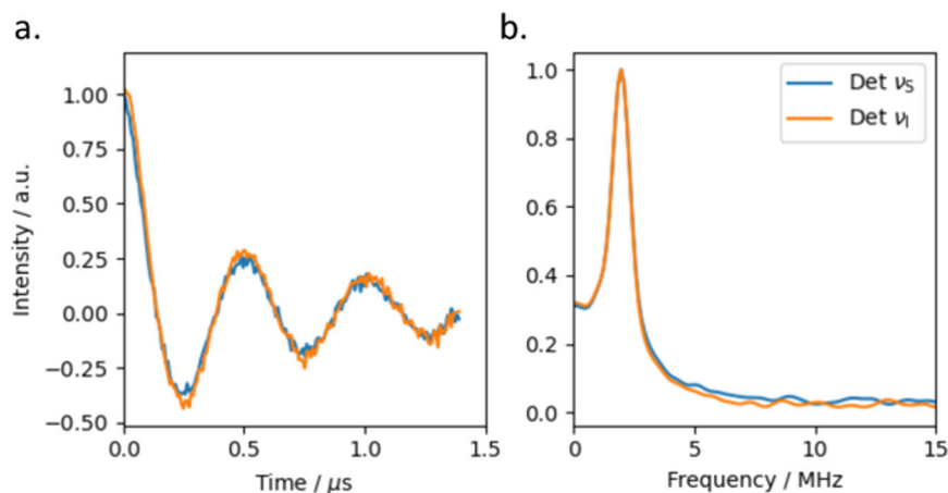
Fig. 4 | 3P-DEER traces for 1. a Background corrected 3P-DEER traces (left). b Corresponding Fourier transforms. DEER traces recorded detecting at \nu_S (9.54 GHz) and pumping at \nu_I (9.69 GHz) (blue) and detecting at \nu_I and pumping at \nu_S (orange). Definition of \nu_I and \nu_S as Fig. 2.
