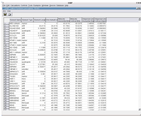
Figure 4: The optical functions presented in tabular form.
