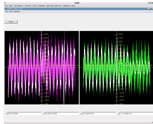
Figure 6: The trajectory tracer.
