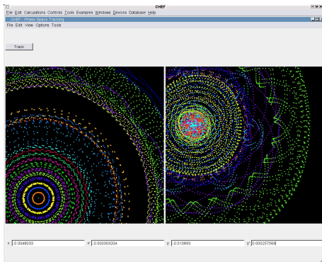
Figure 5: The phase space tracker.
