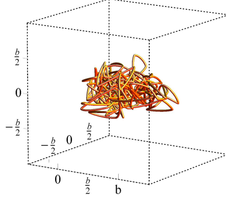
Figure 7.12: 3D configuration of the string with N = 200 and g = 0.3 using D_{\perp}(\lambda) in the interaction. See text.
