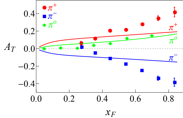
Figure 4.8: x_F dependent SSA in p_\uparrow p \rightarrow \pi X collisions at \sqrt{s} = 19.4 \text{ GeV} [3]. The solid lines are the analytical results in Eq. (4.60)- Eq. (4.62) with c = 2 .
