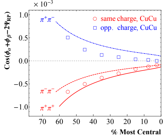
Figure 5.7: Pion azimuthal charge correlations of \text{CuCu} versus the data [6] from STAR at \sqrt{s} = 200\text{GeV} .
