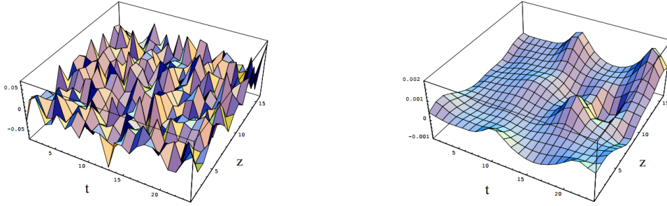
Figure 1.1: Left: typical fluctuations of G\tilde{G} in a lattice simulation with a lattice unit of 0.16 fm. Right: the same fluctuations of G\tilde{G} after 25 cooling sweeps with a lattice unit of 0.14 fm.
