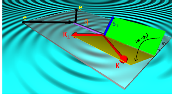
Figure 4.2: The lepton and photon are in the same plane. The angle between the transversely polarized spin s_\perp and this plane is \phi_s . The angle between the transversely spatial momentum K_\perp of the outgoing pion and the plane is \phi .
