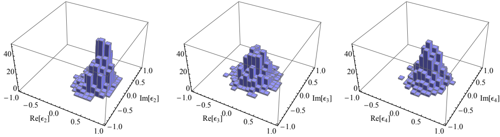
Figure 7.17: 3D Histograms, 1000 random generated strings. N=200 .
