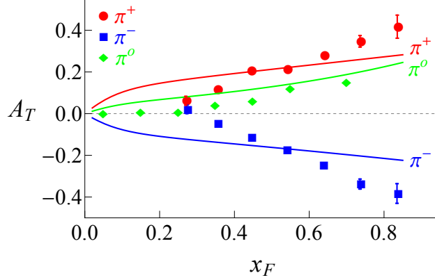
Figure 4.9: x_F dependent SSA in p\uparrow p \rightarrow \pi X collisions at \sqrt{s} = 19.4\text{GeV} [3]. The solid lines are the analytical results in Eq. (4.60)- Eq. (4.62) regulated by using a massive gluon propagator yields the results.
