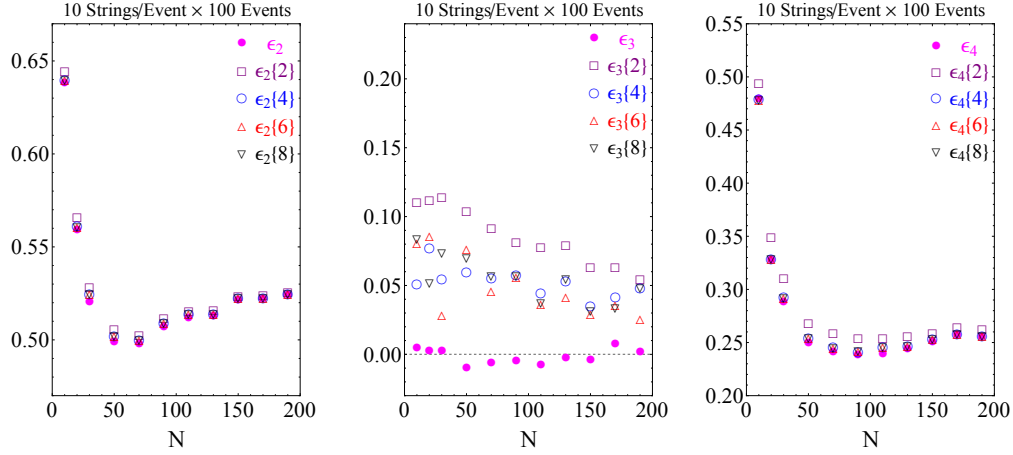
Figure 7.26: Attractive interaction g = 0.3 .
