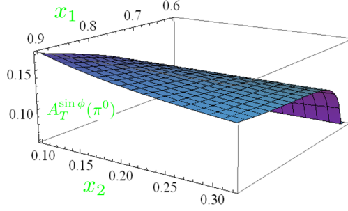
Figure 4.14: SSAs A_T^{\sin\phi}(\pi^0) for x_F = 0.6 .
