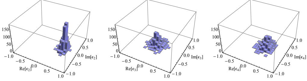
Figure 7.18: 3D Histograms, 1000 random generated strings. N=200 . Attractive interaction g = 0.3 .
