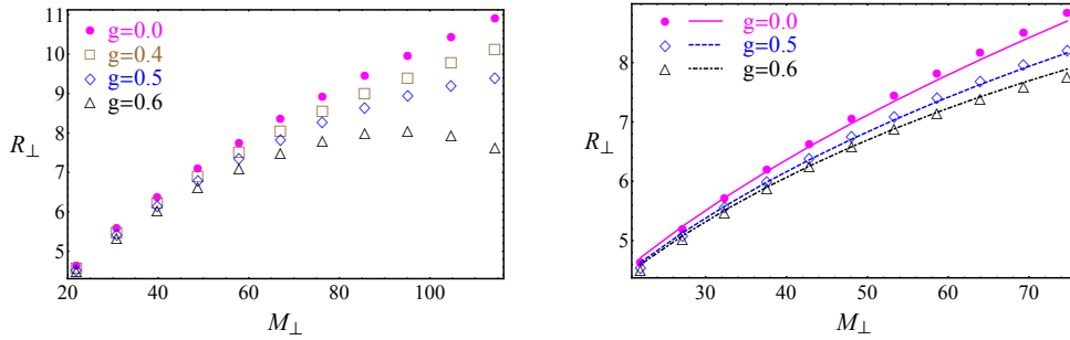
Figure 7.36: Transverse size of the interacting string for N = 500 string bits and attractive self-coupling coupling g versus its mass (left). The solid curves are analytical results (right).
