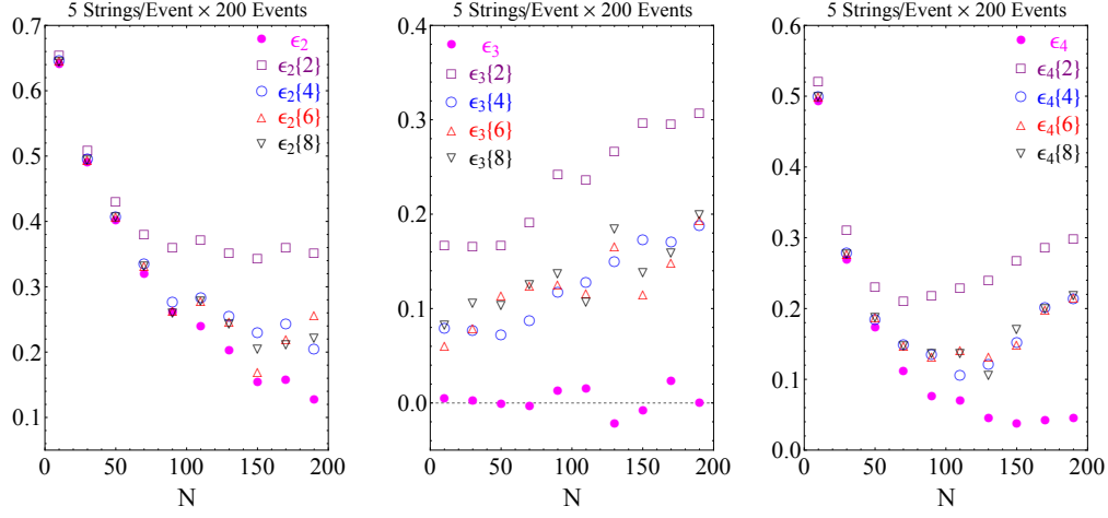
Figure 7.25: Repulsive interaction \tilde{g} = 0.3 .
