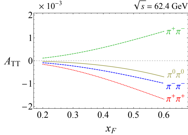
Figure 5.2: Predictions for charged di-jet production in semi-inclusive DSA.
