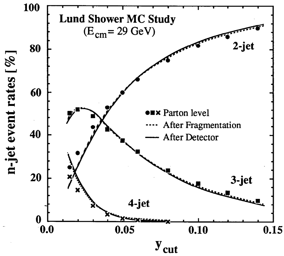
Fig.2 The influence of fragmentation as well as of initial state radiation and detector resolution on n-jet event rates, simulated in model calculations, as a function of y_{cut} .
