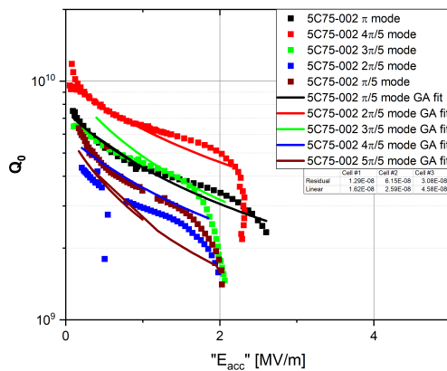
Figure 6: 5C75-J-002 test results for different passband modes at 4.3 K after cavity tuning at room temperature.
