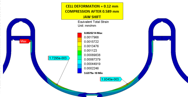
Figure 8: ANSYS tuning simulation of 5C75-J-002 for -0.12 mm wall displacement. Residual cavity shape corresponds to about -150 kHz frequency shift.
