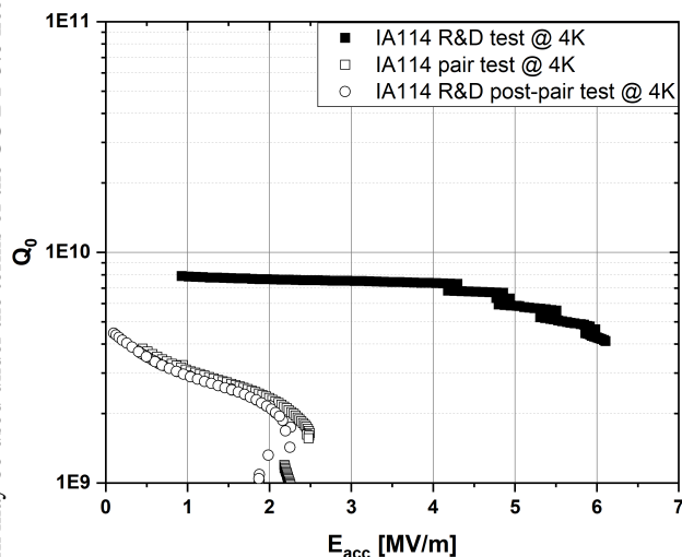
Figure 3: IA114 test results after Nb 3 Sn coating (full squares), after pair assembly (open squares), and after re-assembly with R&D hardware (open circles).
