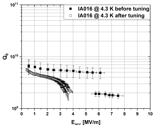
Figure 4: IA016 test result at 4.3 K before and after cavity tuning at room temperature. Note Q-degradation after cavity tuning.
