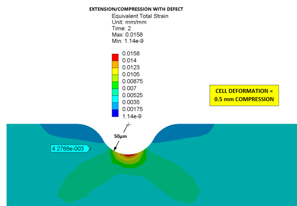
Figure 10: ANSYS tuning simulation of a smooth 50 \mu\text{m} groove located at the equator during -0.5 mm wall displacement. Note the higher strain levels in the pit.
