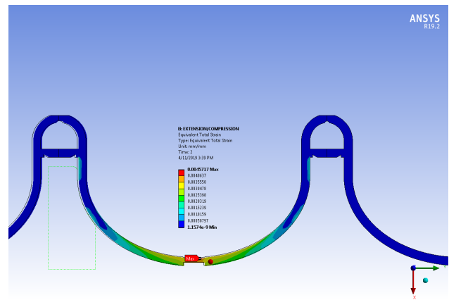
Figure 9: ANSYS tuning simulation of 5C75-J-002 for -0.5 mm wall displacement. Residual cavity shape corresponds to about -600 kHz frequency shift.
