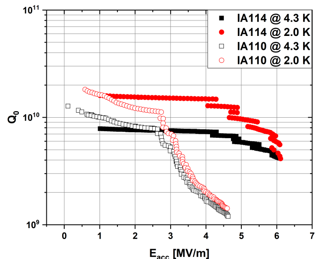
Figure 1: IA114 and IA110 qualification test results at 4 K and 2 K. Discontinuities in Q-curves are due to Q-switches.
