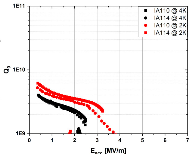
Figure 2: IA110 and IA114 test results after the cavities were assembled into the cavity pair. Note the significant change from qualification tests, Fig. 1.
