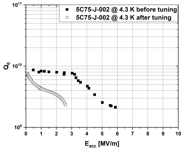
Figure 5: 5C75-J-002 test result at 4.3 K before and after cavity tuning at room temperature. Note Q-degradation after cavity tuning.
