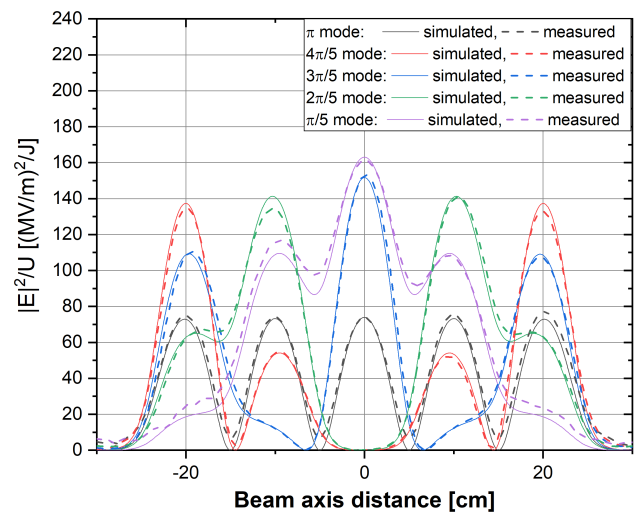
Figure 7: 5C75-J-002 test results for different passband modes at 4.3 K after cavity tuning at room temperature. Passband modes, measured using bead pull technique, were scaled for illustration purposes.
