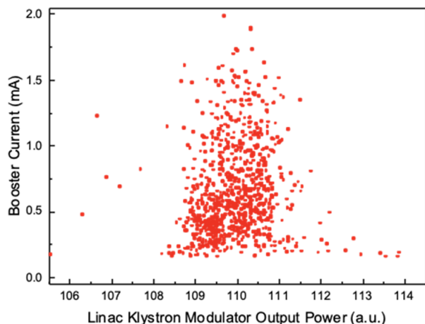
Figure 4: Relation between output power of the modulator and booster current.
