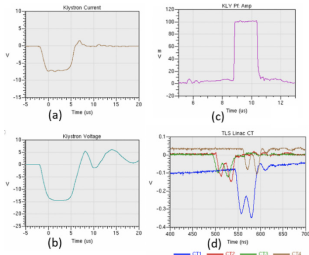
Figure 3: (a) Klystron output current, (b) klystron output voltage, (c) klystron output power and (d) CT1~CT4 waveforms.
