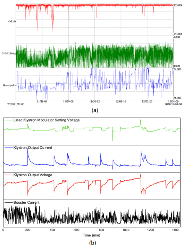
Figure 6: Monitoring the automatic tuning program; (a) one week of operating status, and (b) one day of operating status.
