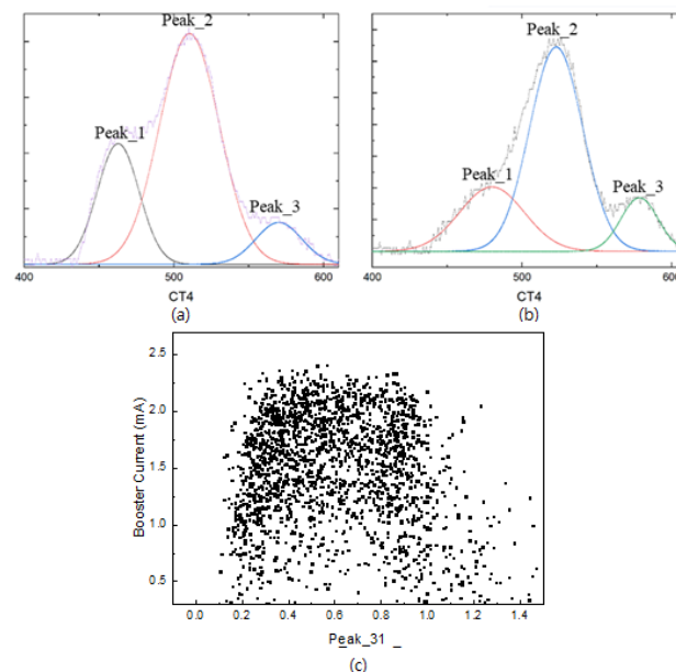
Figure 5: CT4 waveform analysis, (a) state of low output energy, (b) state of high output energy, (c) statistical relation between peak_31 ratio (peak_3 intensity/peak_1 intensity) and booster current output.
