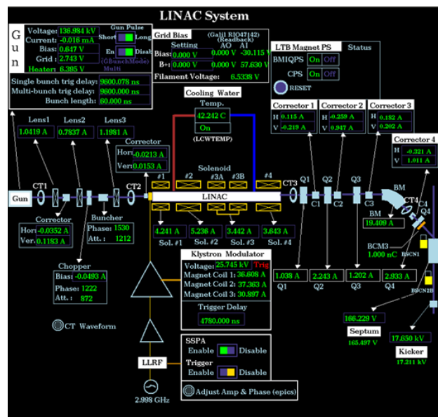
Figure 2: Linear-acceleration section configuration.
