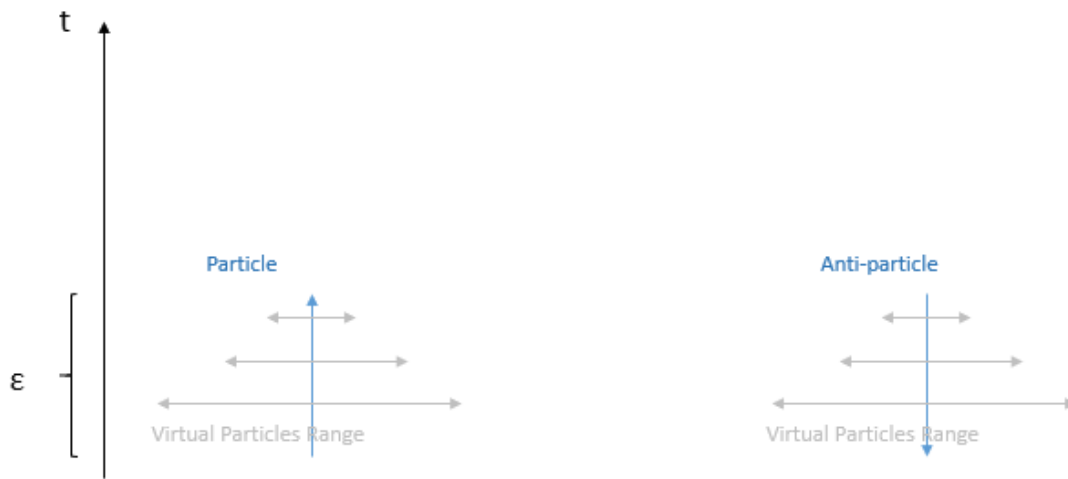
Figure 1: Moving particles in perturbative mode have at a given time a smaller cloud of entangled virtual pairs than anti-particles due to them going back in time (and remembering that neutrinos and anti-neutrinos move quasi at the speed of light. Note the arrow of time, that distinguish this reasoning of reversing the role of particles and anti-particles.
