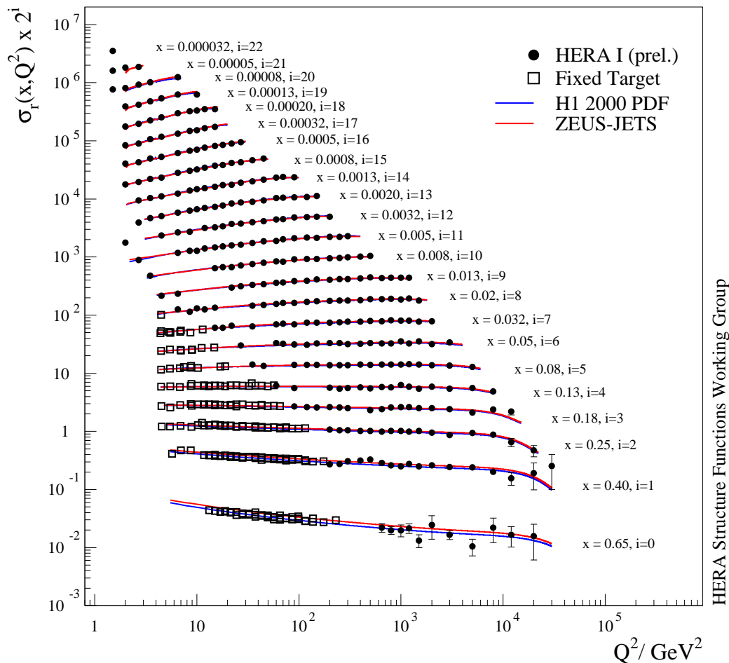
Figure 2. H1 and ZEUS combined neutral current e^+p reduced cross sections [7] (labelled HERA I (prel.)), based on the published HERA I data. The curves are NLO QCD fits as performed by H1 and ZEUS to their own data.
