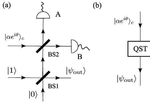
Fig. 2. Quantum state truncation scheme.
