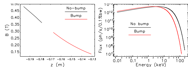
Figure 4: Left: Dipole field along the beam trajectory in the dipole showing only the regions radiating into the HSCU chamber. Right: Photon flux integrated over field regions shown on the left plot.
