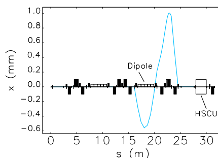
Figure 1: Orbit bump that generates positive orbit angle at the exit of the dipole, which only spans half the sector and has small overall orbit distortion. One lattice sector is shown.
