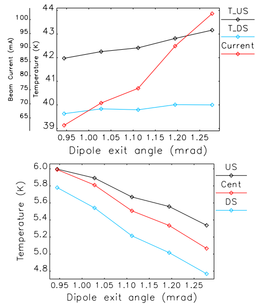
Figure 3: Vacuum chamber temperature (top) and magnet temperature (bottom) as a function of the dipole exit angle. Electron beam current is varied to keep the vacuum chamber temperature approximately constant (also shown on the top plot).
