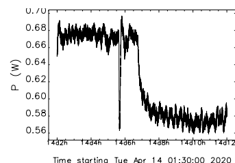
Figure 5: Reduction in heater power required to keep the LHe tank pressure at 760 Torr after the beam was injected into the ring.
