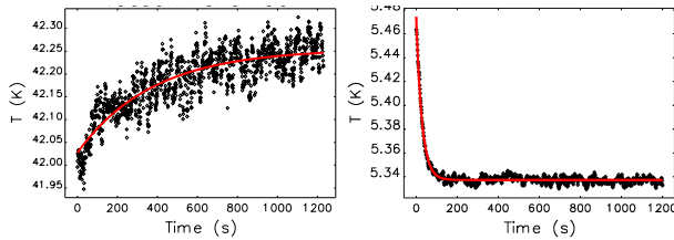
Figure 2: Typical temperature settlement during single scan point measurement. Left – vacuum chamber, right – magnet. Red line shows the exponential fit of the measured (black) points.
