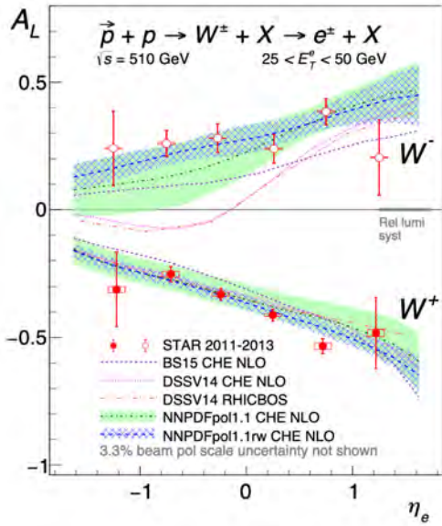
Figure 3: Measured A_L for W^\pm vs. lepton pseudorapidity ( \eta_e ) together with theory expectations (curves and bands). Data shown are combined from 2011, 2012 and 2013 [5].
