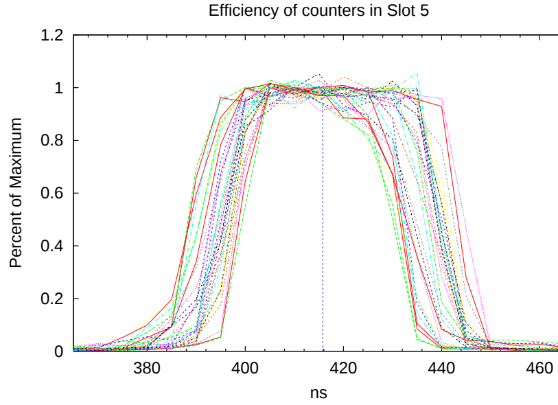
Figure 3.9: Inner muon timing efficiency plateau. The efficiency is a crude estimate based on the number of firings per event, normalized to the peak of each plateau. The dashed line represents the optimal value for the PCOS latch delay. The height of the plateau is approximately 40 ns , which is the width of the latch gate. The different colors represent the 32 channels going into this module.
