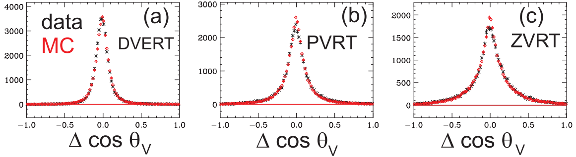
Figure 4.17: We show resolution plots of the distribution of \Delta \cos \theta_V . We show the difference between \cos \theta_V reconstructed using the line-of-flight method on a “blanked” K3\pi sample minus the \cos \theta_V computed from a fully reconstructed sample. The “blanked” pion representing the neutrino is the softest pion. Black is data and red is Monte Carlo. The data and Monte Carlo have been background subtracted using the sidebands illustrated in Figure 4.16. The plots use different primary vertices to compute the line of flight: (a) The DVNUCL vertex, (b) the most detached DVFREE vertex, and (c) A ZVRT vertex chosen to give the D^0 a nominal 0^\circ line-of-flight along the direction of the incident photon.
