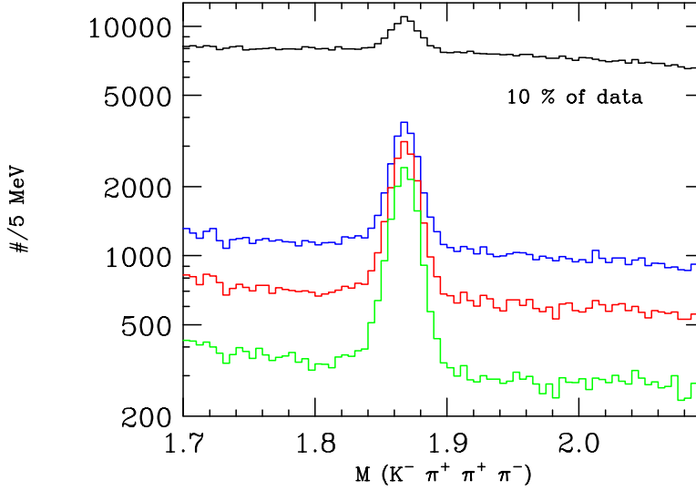
Figure 4.4: Illustration of the effectiveness of Čerenkov cuts in reducing backgrounds to D^0 \rightarrow K^- \pi^+ \pi^+ \pi^- . Note the logarithmic scale. The upper curve has no Čerenkov cuts. The second histogram requires \Delta W_K > 0 . The third requires \Delta W_K > 2 . The fourth histogram requires \Delta W_K > 2 and \Delta W_\pi > -2 . The fitted signal yields in these plots are 15307, 12783, 11699, and 9996 respectively.
