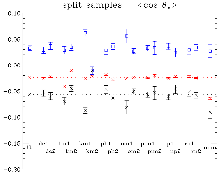
Figure 7.10: \langle \cos \theta_v \rangle for split samples.
