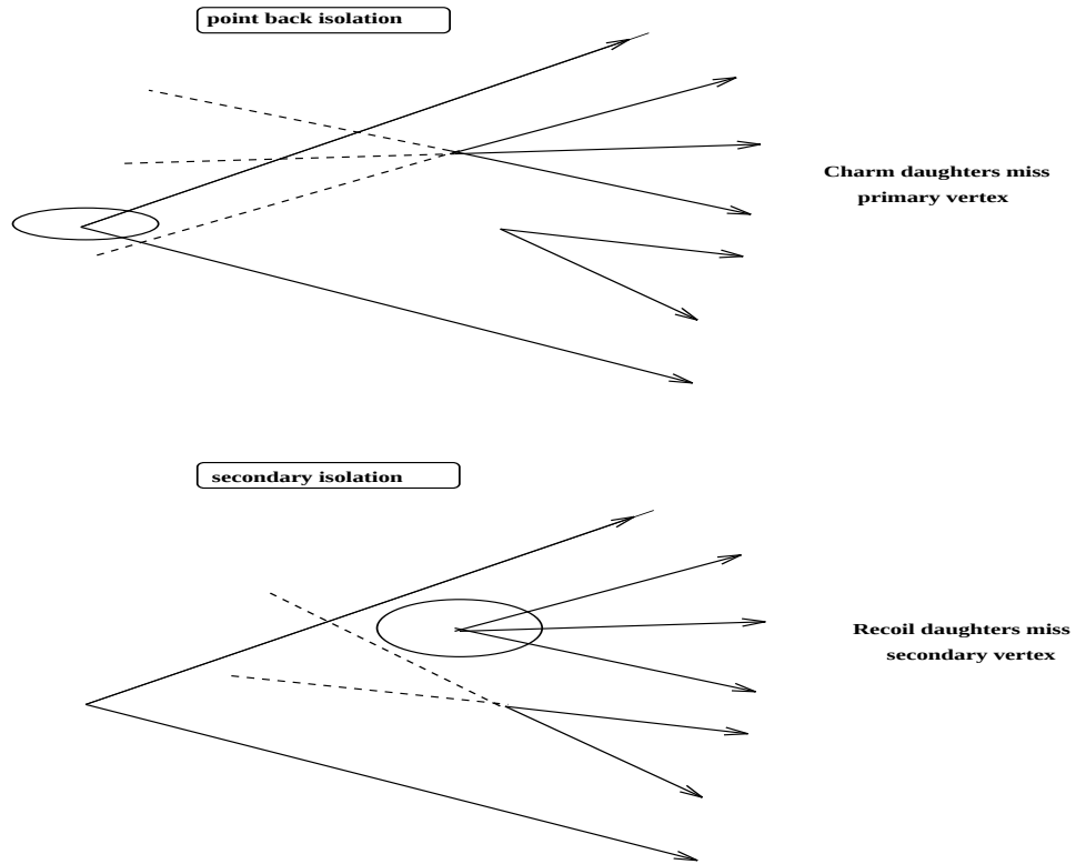
Figure 4.1: Schematic representation of isolation cuts ISOP and ISO2
