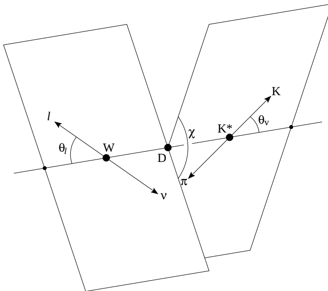
Figure 2.1: Definition of the decay angles \theta_v , \theta_\ell , and \chi
