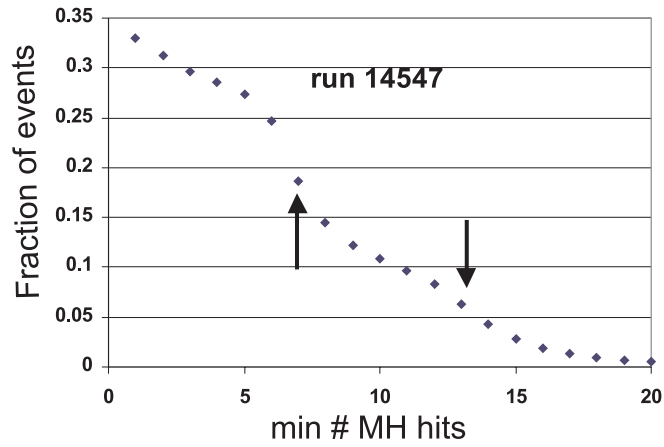
Figure 4.5: We plot the fraction of events in Run 14547 with the number of struck counters in the inner muon system equal to or exceeding the abscissa. A clear “knee” can be seen at 6 or more hits which we attribute to a muon halo track traversing all 6 counter planes that comprise the inner muon system. This knee is rather broad because of range out, wide angle muons that pass wide of the last detector plane, and muons that fire adjacent counters.
