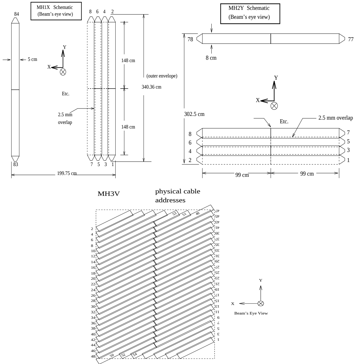
Figure 3.7: Inner Muon array schematics. The schematics for MH1Y, MH2X and MH3U are similar to MH1X, MH2Y and MH3V respectively. The MH3 detectors are each 10 cm wide.
