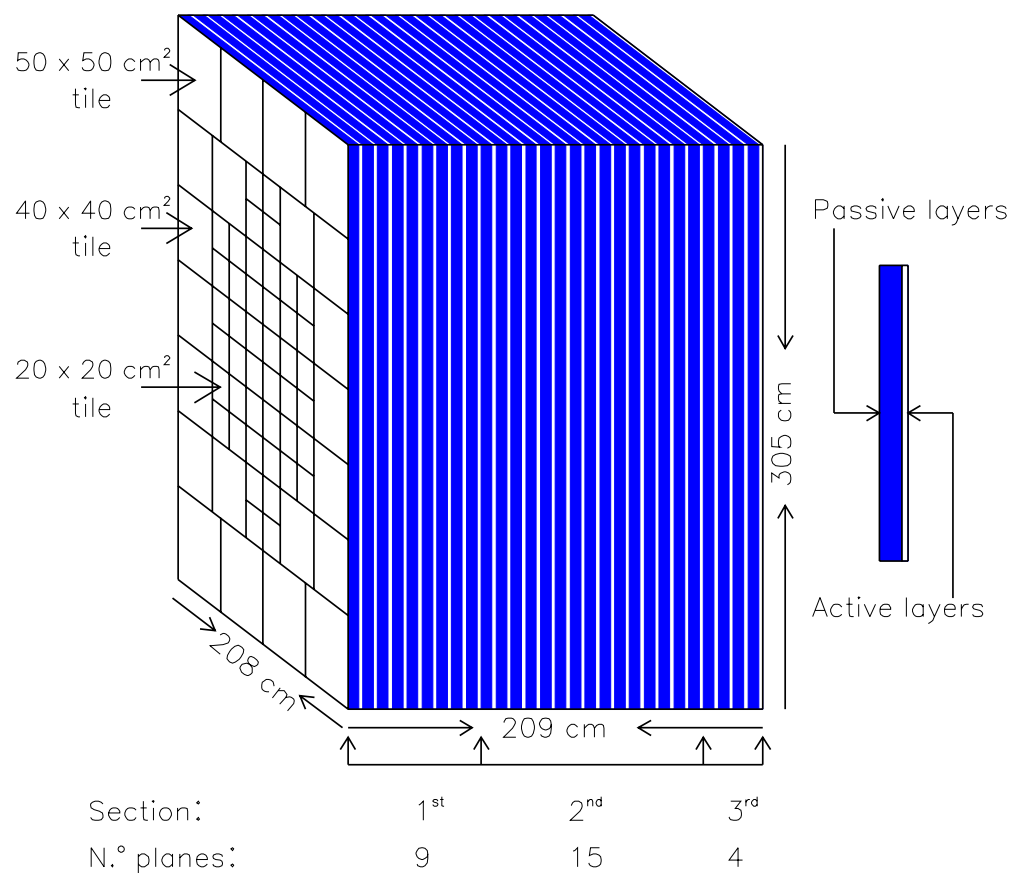
Figure 3.6: HC schematic .
