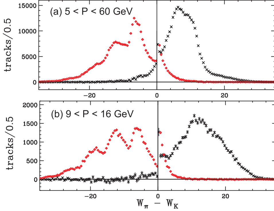
Figure 4.3: The log likelihood difference W_\pi - W_K distribution obtained from background subtracted kaons and pions from golden mode charm signal shown in Figure 4.2. The pion distributions were rescaled to have the same area as the kaon distributions. Plot (A) is for tracks with momenta in the range 5 < P < 60 GeV/ c . Plot (B) is for tracks with momenta in the range 9 < P < 16 GeV/ c . There are off-scale spikes in the 0 bin consisting of 20,000 and 4,500 events for Plots (A) and (B).
