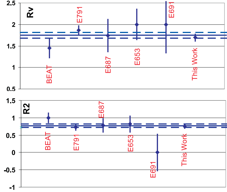
Figure 9.1: Experimental data on r_v and r_2 . Horizontal lines indicate the average values of the form factor ratios including this measurement along with their errors. The weighted average values are r_v = 1.754 \pm 0.064 and r_2 = 0.773 \pm 0.052 . The confidence level that all six r_v measurements are consistent is 58%. The confidence level that all six r_2 measurements are consistent is 48%.
