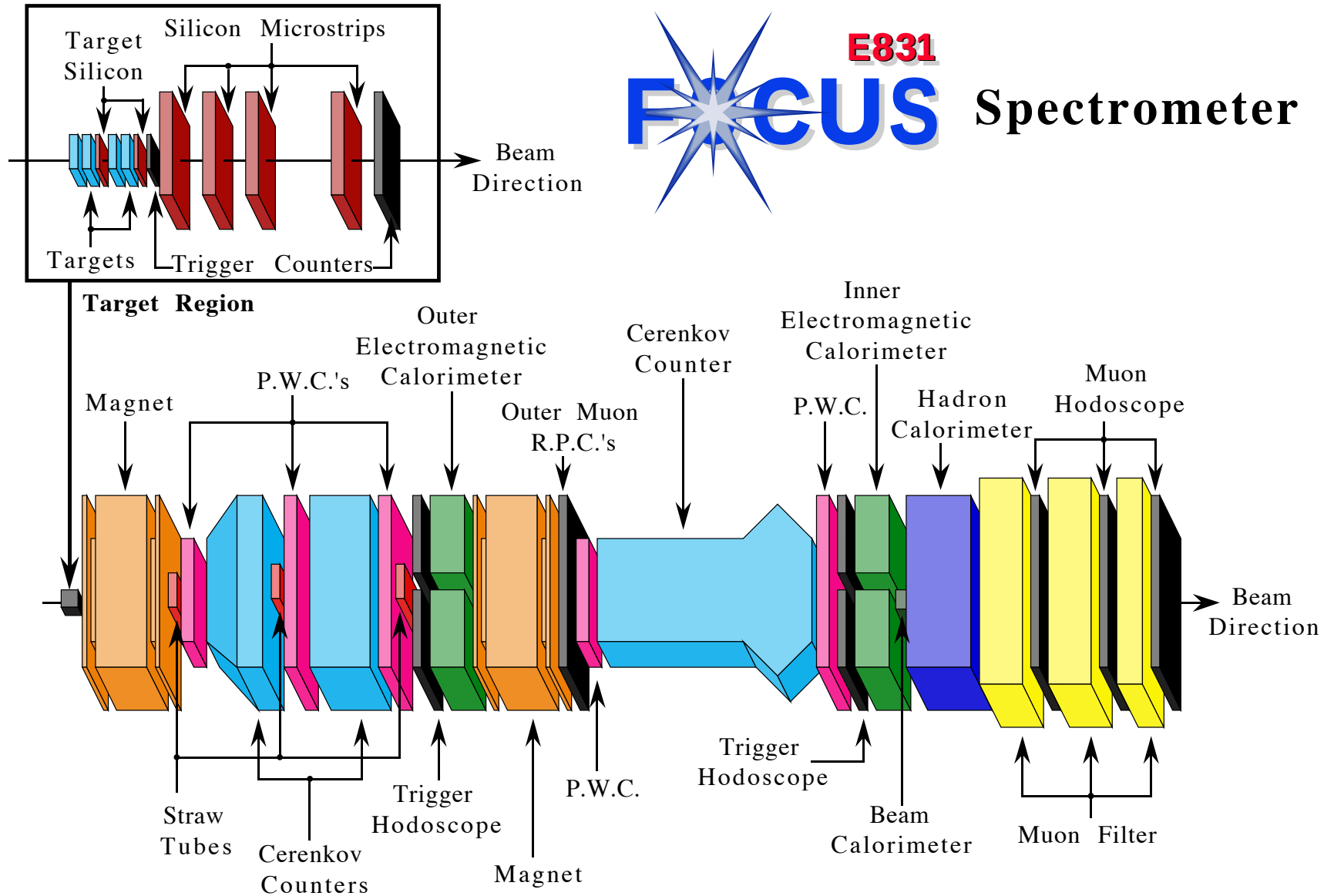
Figure 3.3: FOCUS spectrometer. In the upper left, the target region is shown.
