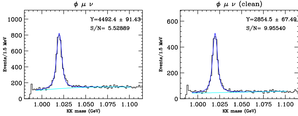
Figure 1.4: \phi mass for D_s^+ \rightarrow \phi \mu^+ \nu_\mu candidates. The plot on the left has cuts which are about as loose as might be possible for a form factor measurement. These are: \text{DCL} > 1\% , \ell/\sigma > 5 , \text{Iso2ex} < 0.1 , IMU only, minimum kaonicity > 3 , the D \rightarrow K^- K^+ \pi^+ normalized mass is > 2\sigma away from the true D^+ and D_s^+ masses, and \mu\text{-misspl} < 2 . For the plot on the right, additional cuts are applied: \text{DCL} > 10\% , and \text{CL}_\mu > 0.05
