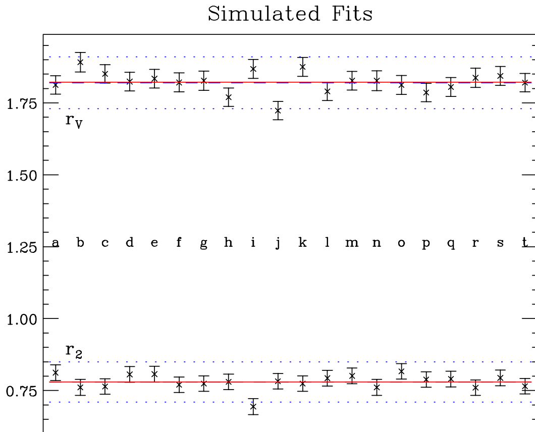
Figure 6.1: Fits of simulated data. Black points are the individual fit results with their errors. The red lines are the averages of these fits, and dashed blue lines are the input values. These are hidden underneath the red line but are centered between the dotted blue lines.
