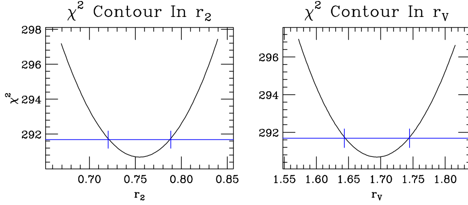
Figure 7.3: \chi^2 contours for the baseline fit. The blue cross-hairs are one unit above the fit minimum, and 1\sigma to the left and right. If the contour is truly parabolic, and the fit parameters are not strongly correlated, it will intersect at these points. It evidently does. According to the fitter, there is a 21% anti-correlation between r_v and r_2 , which is not severe.
