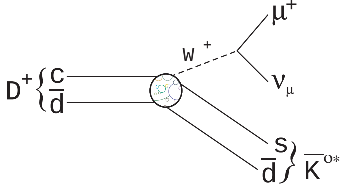
Figure 1.1: quark-level diagram of the semileptonic decay D^+ \rightarrow \bar{K}^{*0} \mu^+ \nu_\mu .
