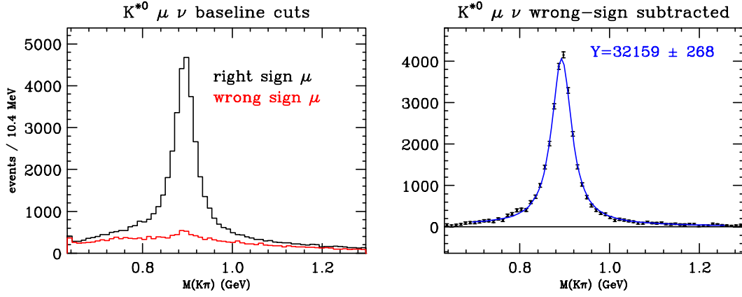
Figure 7.1: D^+ \rightarrow \bar{K}^{*0} \ell^+ \nu_\ell signal with baseline cuts. The plot on the right is wrong-sign subtracted, and fitted with a Breit-Wigner (non-relativistic spinless) convoluted with a 5 MeV-wide Gaussian plus a linear background. The fitted signal yield is 32159 \pm 268 events.
