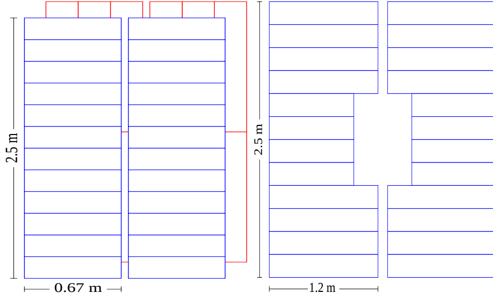
Figure 3.10: H \times V and OH schematic
