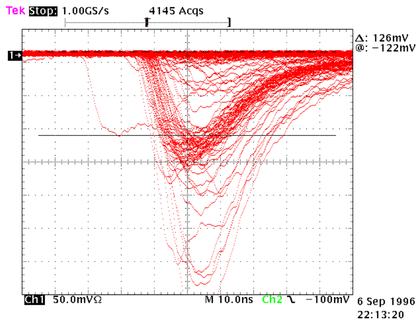
Figure 3.8: Pulses from muons in the inner muon detectors. This is a collection of electronic pulses at the input to the discriminators. There is a main clustering of pulses which represent genuine muon hits. The average height of these pulses were measured and used to tune the high voltage setting for the given PMT. For this detector, the minimum pulse height was roughly 126 mV. The discriminator voltage would have been set to about half this value.
