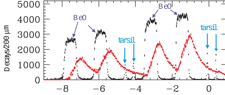
Figure 3.2: Z distribution for the primary and secondary vertices for the background subtracted Golden mode charm. The black points are the positions of the charm production vertices, and red points correspond to the charm decay vertices. The BeO segmented target and target silicon detector planes are evident. This also illustrates the way the segmented target configuration greatly increases the number of charm decays out of the target material.
