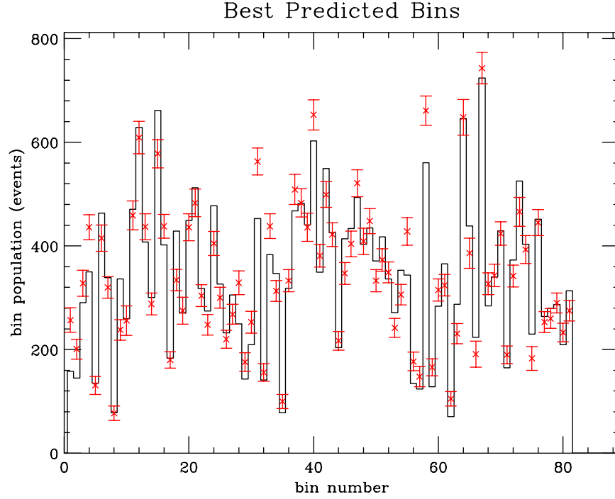
Figure 7.2: Bin populations and predictions for baseline fit. 3 bins in \cos \theta_V , \cos \theta_\ell , Q^2/Q_{\max}^2 , and |\chi| for a total of 81 bins. The red points with error bars are the observed bin populations. The black lines are the best-fit bin predictions.
