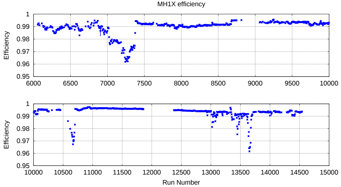
Figure 4.6: The average efficiency of the MH1X array based on the fraction of times this array fires in events where all other muon planes fire. The efficiency of all other planes is very comparable to the efficiency of this plane. The 2% inefficiency dip near 7250 was due to a slight shift in the latch timing. We corrected this timing immediately after discovering the problem — thus restoring the efficiency to its original level.
